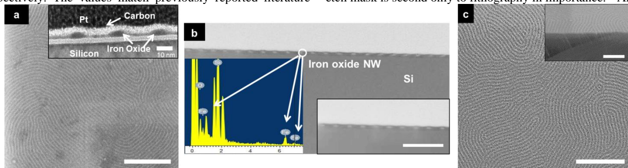
Fig. 3 (a) Top-down SEM image of \text{Fe}_3\text{O}_4 nanowire array after UV/ \text{O}_3 treatment. Inset in (a) shows cross section TEM of \text{Fe}_3\text{O}_4 nanowires/substrate interface. (b) EDX spectrum of \text{Fe}_3\text{O}_4 nanowire array and HAADF image and inset show uniformity and regularity of \text{Fe}_3\text{O}_4 nanowire array. (c) Top-down SEM image of \gamma\text{-Al}_2\text{O}_3 nanowire arrays after UV/ \text{O}_3 treatment. Inset in (c) shows cross-section SEM view of \gamma\text{-Al}_2\text{O}_3 nanowires. Scale bars are 500 nm in (a) and (c) and represent 100 nm in (b).
