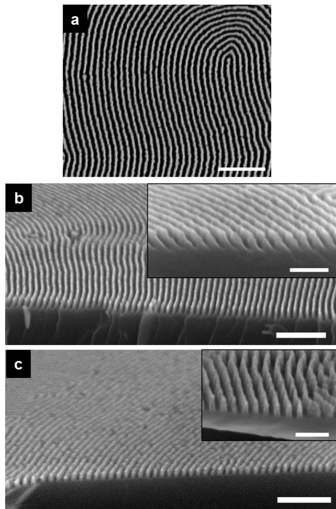
Fig. 8 (a) Top-down SEM image of pattern transfer of \gamma\text{-Al}_2\text{O}_3 hardmask nanowires on planar Si generating Si nanofins. (b) Cross-section SEM view of sample (a) after 1 minute and 30 seconds of Si etching. (c) Cross-section SEM view of Si nanofins over large area following 2 minutes of Si etching with \gamma\text{-Al}_2\text{O}_3 as hardmask. Inset in (c) reveals the vertical profile and uniform nature of the nanofins. Main scale bars are 250 nm while inset scale bars represent 100 nm.
