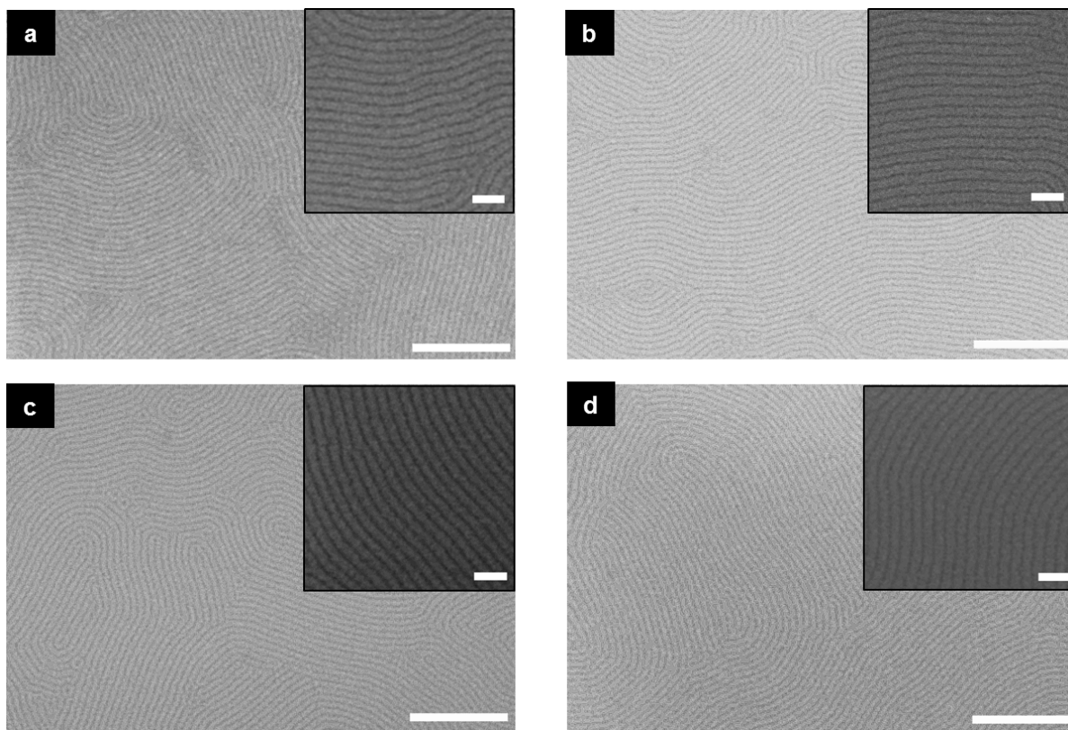
Fig. 1 PS- b -P4VP BCP films were spin coated from a 0.5 wt % solution on to acetone degreased Si substrates. Top-down SEM images are shown in (a)-(d) after solvent vapor annealing with chloroform at room temperature ( \sim 290 K) of a 24 nm thick PS- b -P4VP BCP film for (a) 30 minutes, (b) 1 hour, (c) 2 hour and (d) 3 hours respectively. Note films were exposed to ethanol vapors following solvent vapor annealing to create porous structures. Scale bars are 500 nm, while inset scale bars are 100 nm.
