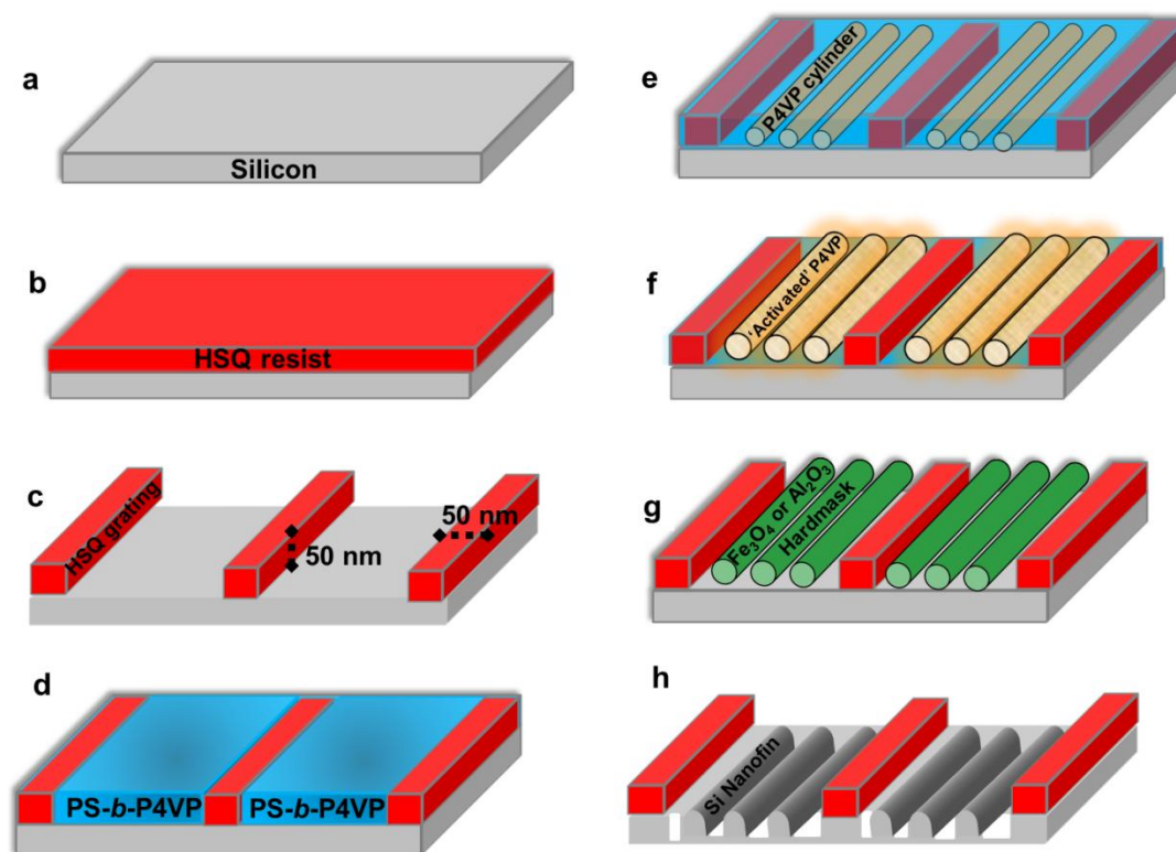
Scheme 1. Overall process flow enabling Si nanofins via an enhanced metal oxide pattern transfer. (a) Si substrate (b) Uniform HSQ resist material spin coated (c) Electron beam lithography used to define 50 nm HSQ gratings at different pitches (see experimental) (d) PS- b -P4VP BCP spin coated (e) Solvent vapor annealing of BCP film in chloroform vapors at room temperature producing P4VP cylinders in plane (f) Film exposed to ethanol vapors to form ‘activated’ porous P4VP nanodomains (g) Iron or aluminium oxide formed via inclusion and UV/ozone treatment (h) Pattern transfer to underlying Si forming aligned Si nanofins.
