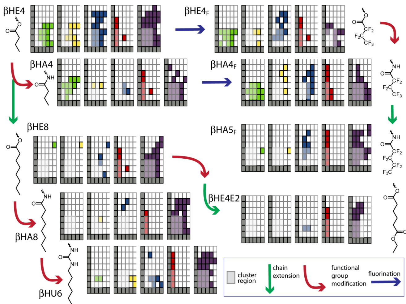
Figure 7: Activity grids of single-chain derivatives related by incremental structural changes.
