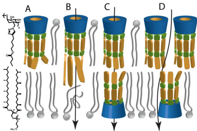
Fig 9: Candidate structures of potential conducting states.
