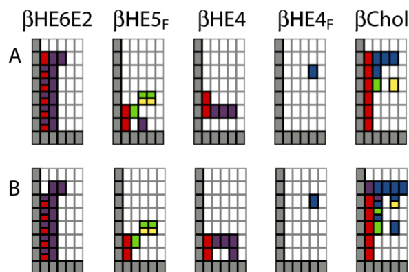
Figure 4: Activity grid methodology.
