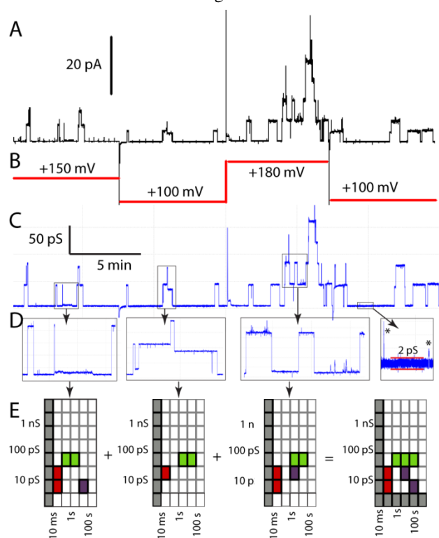
Figure 3: Processing of experimental data to produce an activity grid.
