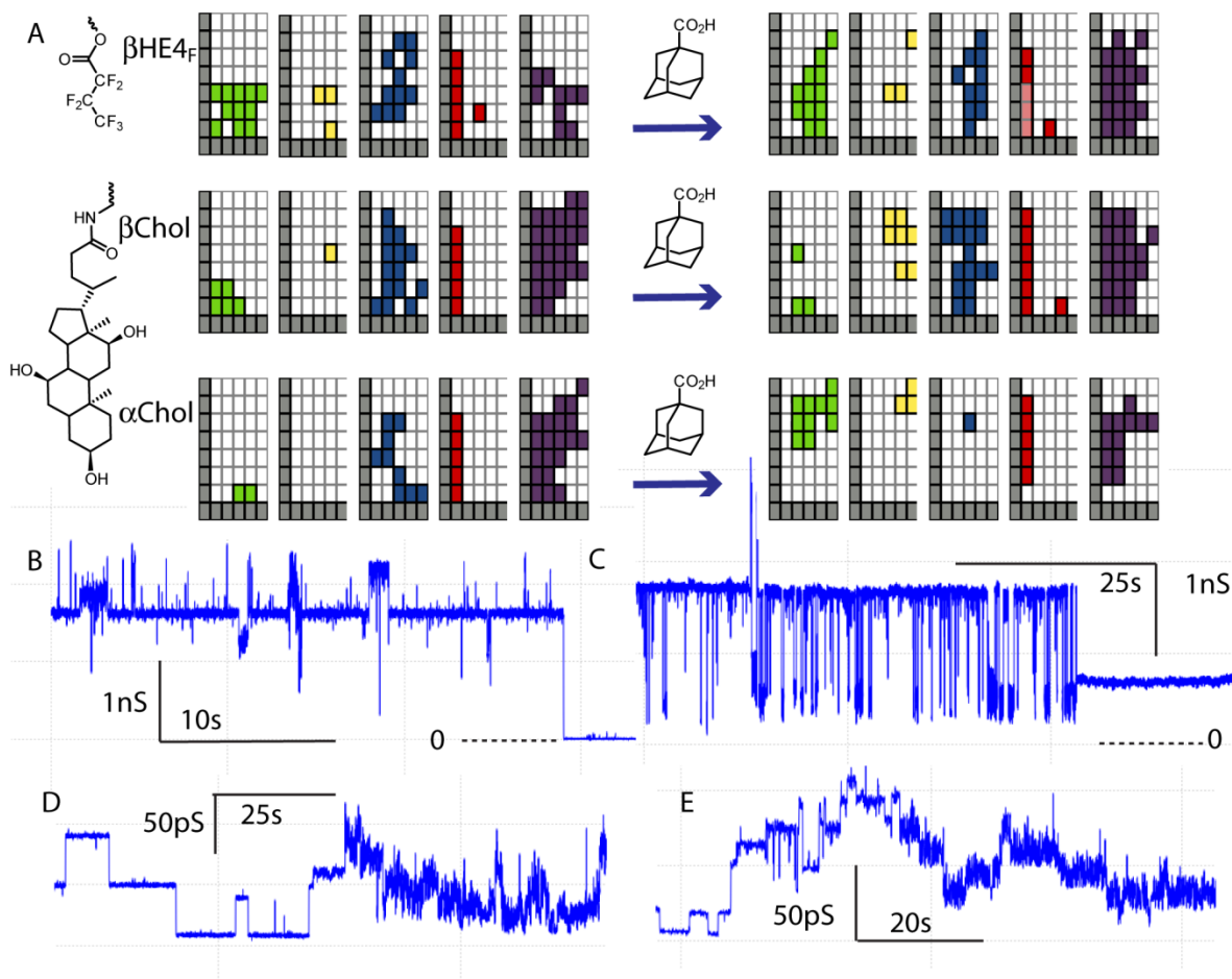
A: activity grids of membrane conductance before and after addition of adamantane carboxylic acid (grids sum several experiments with various concentrations and electrolytes); B: Example of high-conductance openings by \beta -Chol (2 mol%) with added adamantane carboxylic acid (2 mol % in diPhyPc; 1M CsCl); C: Example of high-conductance flicker openings by \beta -HE4F (3.3 \mu M in electrolyte) with added adamantane carboxylic acid (0.28 mM) and \beta -cyclodextrin (7 mM; 1M CsCl; diPhyPc); D: Example of low-conductance events by \beta -HE4F (3.3 \mu M in electrolyte) with added adamantane carboxylic acid (0.28 mM; 1M CsCl; diPhyPc); E: Example of low-conductance events by \beta -HE4F (12 \mu M in electrolyte) with added adamantane carboxylic acid (0.33 mM; 1M NaCl; diPhyPc).
