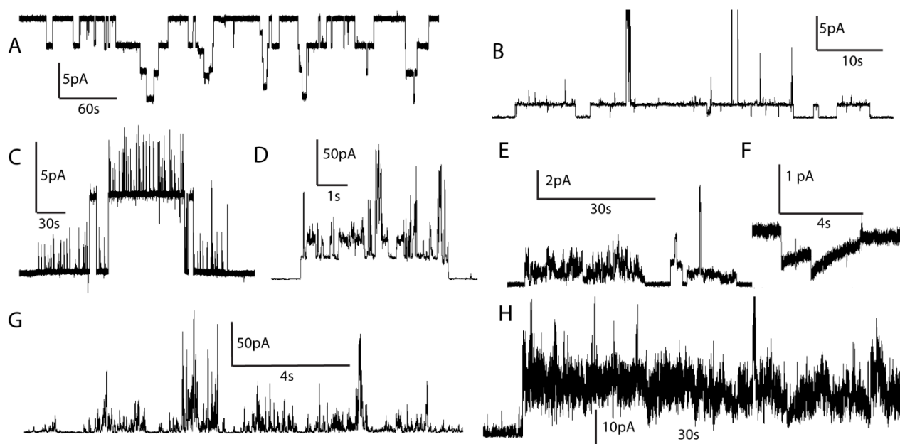
Figure 1: Examples of conductance behaviours of cyclodextrin ion channels a
