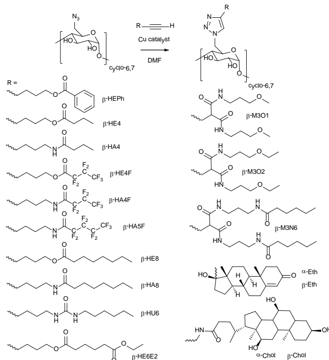
Scheme 1: Synthesis and structures of cyclodextrin ion channels prepared a .
