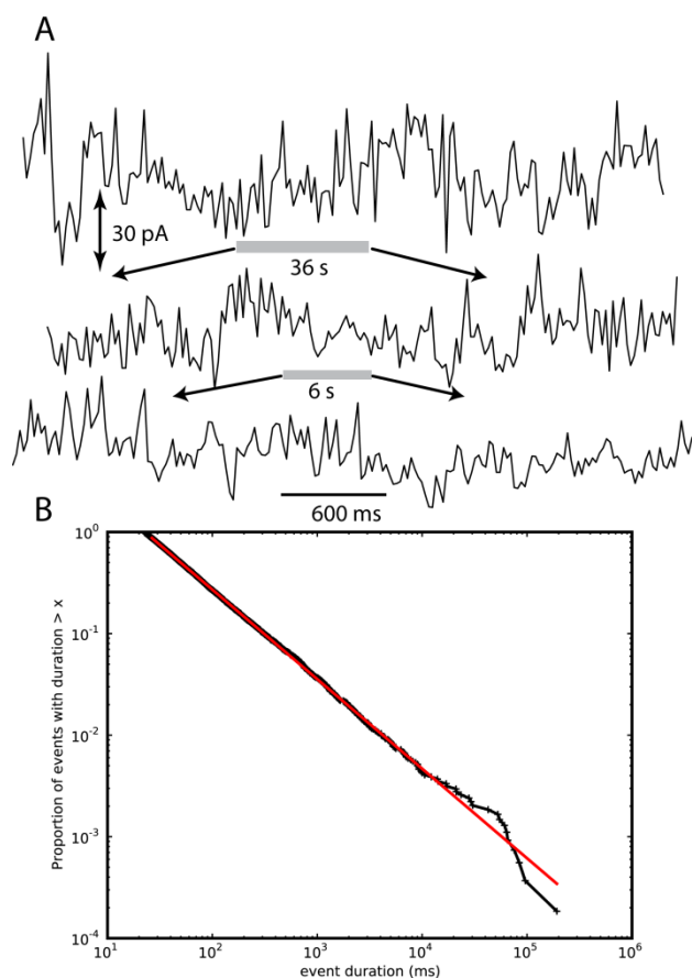
A: current-time record (diPhyPC; 1M CsCl; -100 mV) over three time spans of the same section processed to show 1000 data points in the width displayed. B: cumulative distribution function of “open durations” above a threshold of -60 mV for the same data.
