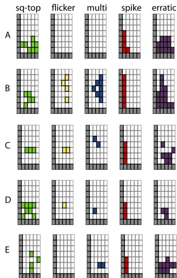
Figure 5: Activity grids for different methods of introduction of \beta -HE4F (diPhyPC, 1M CsCl)
