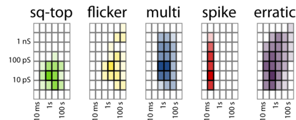
Figure 6: Summary of activity for the entire dataset.
