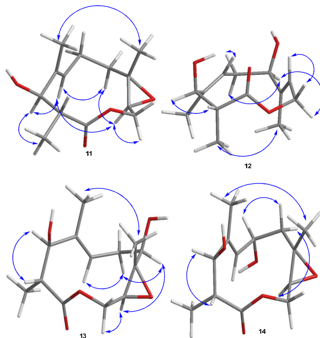
Figure 3. MM2 minimized models with decisive nOe correlations for compounds 11-14 .
