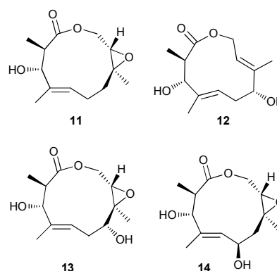
Figure 2. Metabolites isolated in mutasynthesis.
