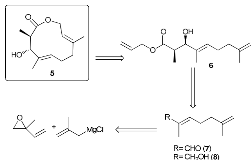
Scheme 1. Retrosynthetic analysis of lactone 5 .
