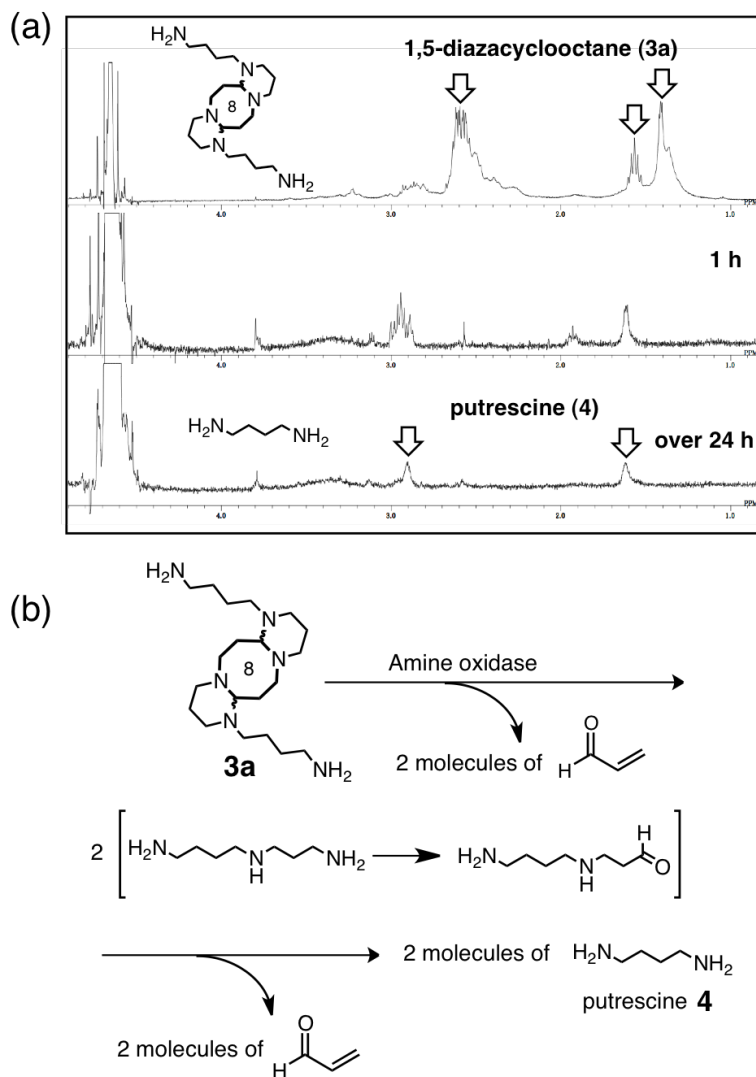
Fig. 2 Oxidation of the 1,5-diazacyclooctane 3a with the serum amine oxidase. (a) The reaction was performed in PBS- d at 37 °C, pH 7.2, using 10 \mu M 3a and 3.8 units bovine serum amine oxidase and was directly monitored using ^1\text{H} NMR techniques. Diazacyclooctane 3a was gradually transformed into the putrescine 4 over 24 h. Lower signal-to-noise ratios of the spectra in the process of the reaction is due to the production of other insoluble polymeric products, e.g., eight-membered polymers. (b) Possible reaction mechanism for the enzyme-catalyzed oxidation of the diazacyclooctane 3a and the production of 4 molecules of acrolein.
