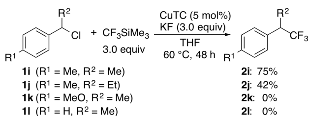
Scheme 2 Copper-catalyzed trifluoromethylation of secondary benzylic chlorides ( 1 ).
