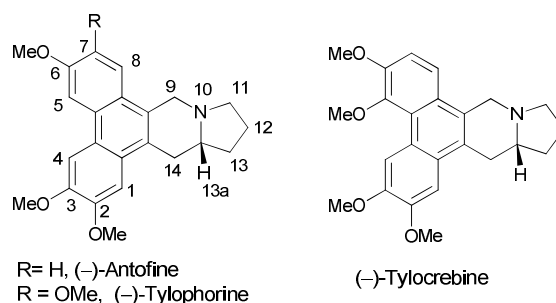
Figure 1. Naturally occurring phenanthroindolizidines.
