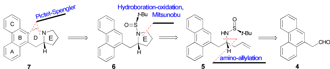
Scheme 1. Retrosynthetic Analysis of Phenanthroindolizidine.
