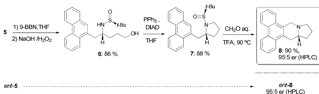
Scheme 3. Synthesis of Phenanthroindolizidines 7 and ent - 7 .
