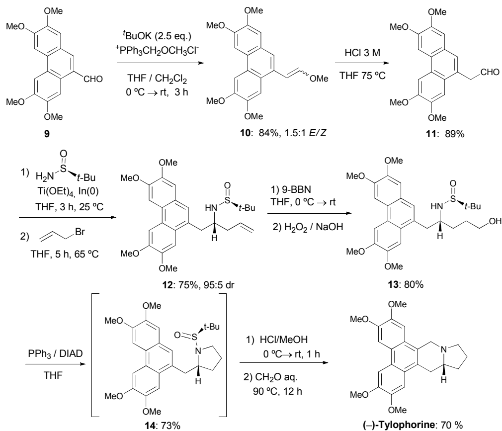
Scheme 4. Synthesis of (-)-Tylophorine.
