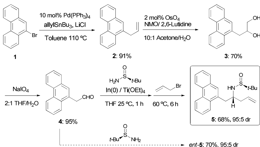
Scheme 2. Synthesis of Homoallylsulfonamines 5 and ent - 5 .
