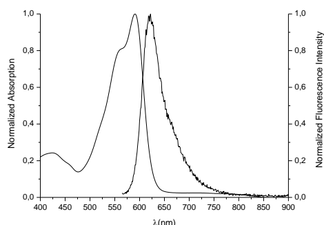
Figure 1. Normalised absorption and fluorescence ( \lambda_{\text{ex}} = 555 \text{ nm} ) spectra of probe P4 in acetonitrile ( c = 1.0 \times 10^{-5} \text{ mol dm}^{-3} ).
