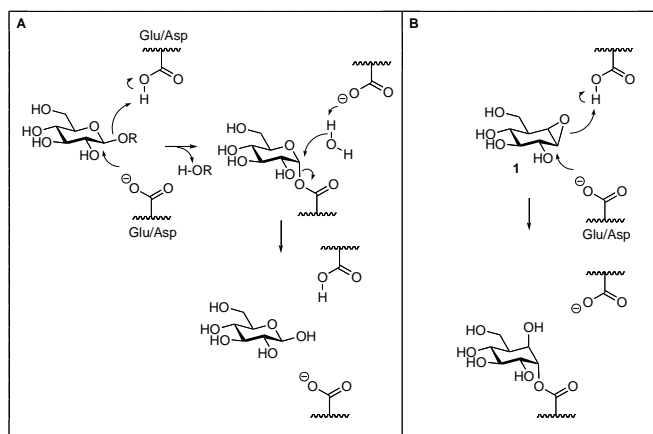
Figure 1. Mechanism of retaining \beta -exoglucosidase-mediated hydrolysis of \beta -glucosidic linkages (A) and mechanism-based, covalent and irreversible inhibition of \beta -glucosidases by the natural product, cyclophellitol 1 (B).
