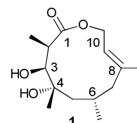
Fig. 1. Structure of compound 1
