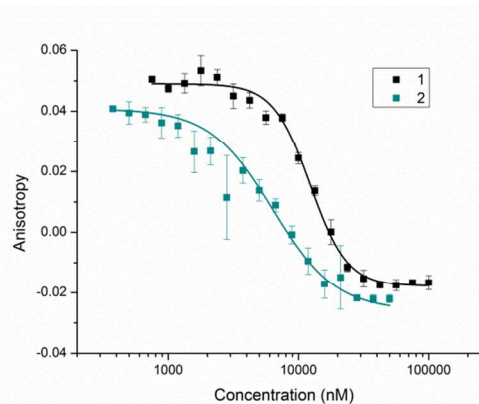
Figure 2 Fluorescence anisotropy competition curves for the inhibition of the p53/hDM2 interaction by the monovalent trimer 1 (black) and the divalent trimer 2 (blue) in assay buffer (40 mM phosphate pH7.5, 200 mM NaCl, 0.02 mg/ml BSA). hDM2 and FITC-p53 were added to a dilution series of the mimetics to give final concentrations of 154.2 and 54.5 nM, respectively.
