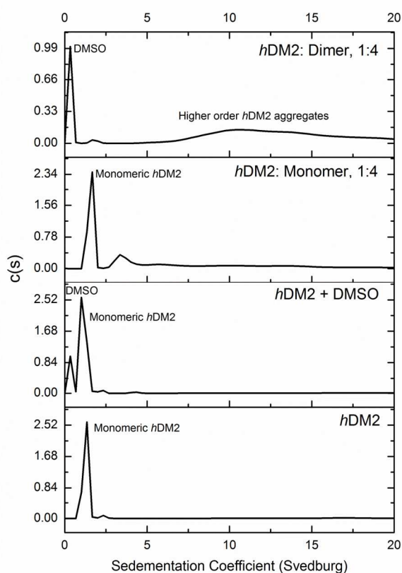
Figure 5 Analytical ultracentrifugation analysis of hDM2 in the presence of monomer 1 and dimer 2 at a 1:4 concentration ratio. Samples were prepared in 40 mM phosphate buffer, 200 mM NaCl and 5% DMSO where appropriate. Samples were centrifuged at 48000 rpm and sedimentation coefficients calculated.
