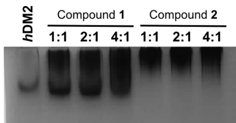
Figure 4 hDM2 analysed by native PAGE in the presence of increasing equivalent of both the monovalent ligand 1 (left) and divalent ligand 2 (right) run in 25 mM Tris buffer pH 8.6, 190 mM glycine. Bands were visualised with Coomassie staining.
