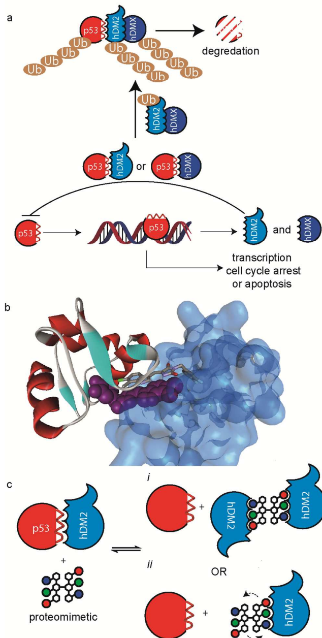
Figure 1. Multivalent interactions of p53 and hDM2 (a) overview of p53 signalling pathway illustrating how hDM2(X) dimerisation enhances ubiquitination of p53 (b) x-ray structure of a small molecule inducer of hDM2 dimerisation (PDB ID: 3VBG). (c) schematic depicting possible consequences of multivalent inhibition of p53/hDM2 (i) inhibition enhances hDM2 dimerization by additional intermolecular hDM2 contacts or (ii) proximity of additional ligand enhances affinity through more rapid association upon displacement of bound ligand.
