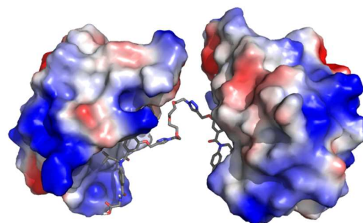
Figure 3 – Molecular modelling of compound 2 ; proposed binding mode of compound 2 in the p53 binding cleft of two hDM2 molecules (PDB ID: 1YCR).
