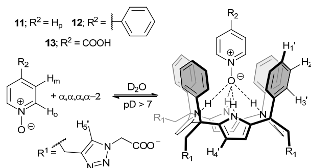
Figure 3. Equilibrium involved in the formation of the inclusion complexes PNO- \alpha,\alpha,\alpha,\alpha - 2 and proposed structure for the binding geometry.
