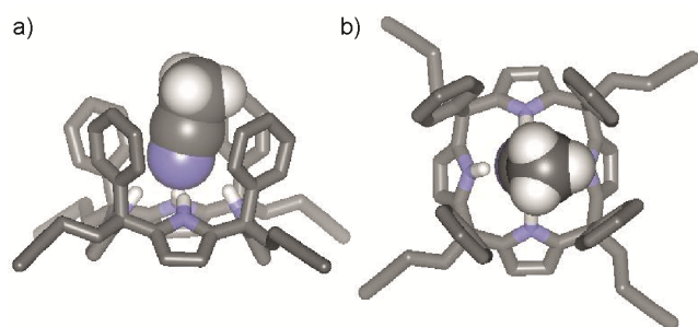
Figure 2. a) Side view and b) top view of the X-ray structure of the aryl extended calix[4]pyrrole \text{CH}_3\text{CN}-\alpha,\alpha,\alpha,\alpha - 3 . For clarity, non-polar hydrogen atoms have been omitted. The included acetonitrile molecule is shown in CPK representation.
