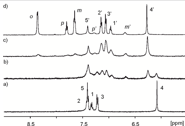
Figure 4. Selected downfield regions of the 1 H NMR spectra (400 MHz, D 2 O adjusted to pD=7.6 with NaOD, 298 K) acquired during the titration of calix[4]pyrrole \alpha,\alpha,\alpha,\alpha - 2 (1 mM) with incremental amounts of 11 . a) \alpha,\alpha,\alpha,\alpha - 2 ; b) \alpha,\alpha,\alpha,\alpha - 2 + 0.6 eq. 11 ; c) \alpha,\alpha,\alpha,\alpha - 2 + 1.1 eq. 11 ; d) \alpha,\alpha,\alpha,\alpha - 2 + 3.4 eq. 11 . Primed letters and numbers correspond to proton signals in the encapsulation complex 11 - \alpha,\alpha,\alpha,\alpha - 2 . See Figure 3 for proton assignment and SI for the analogous titration with 13 .
