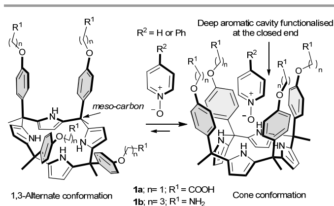
Figure 1. The \alpha,\alpha,\alpha,\alpha -isomers of aryl-extended calix[4]pyrroles undergo a conformational change from the 1,3-alternate conformation to the cone conformation when binding with guests capable of establishing H-bonds.
