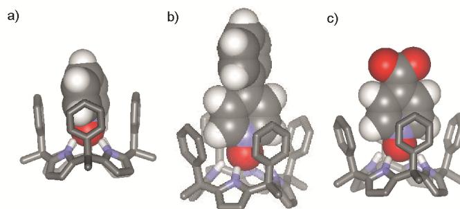
Figure 6. SCIGRESS (v 3.0.0, Fujitsu Ltd.) energy minimized (MO-G PM6 in water) structures of the inclusion complexes of the N -oxides with \alpha,\alpha,\alpha,\alpha-2 : a) 11 ⊂ \alpha,\alpha,\alpha,\alpha-2 ; b) 12 ⊂ \alpha,\alpha,\alpha,\alpha-2 ; and c) 13 ⊂ \alpha,\alpha,\alpha,\alpha-2 . The meso -alkyl chains of the receptor were modelled as methyl groups. For clarity, only the polar hydrogen atoms of the receptor are shown and the included guest is represented as CPK model.
