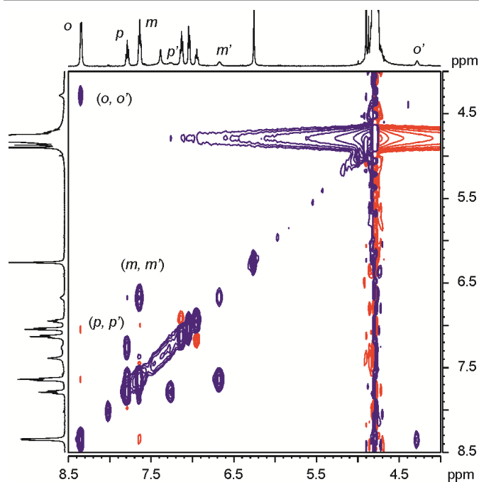
Figure 5. Selected region of ROESY 1 H NMR spectrum of complex \mathbf{11}\subset\alpha,\alpha,\alpha,\alpha - 2 in the presence of free 11 in excess. The cross-peaks resulting from chemical exchange between protons of free and included 11 are indicated. Primed letters correspond to signals of the protons in the complex.
