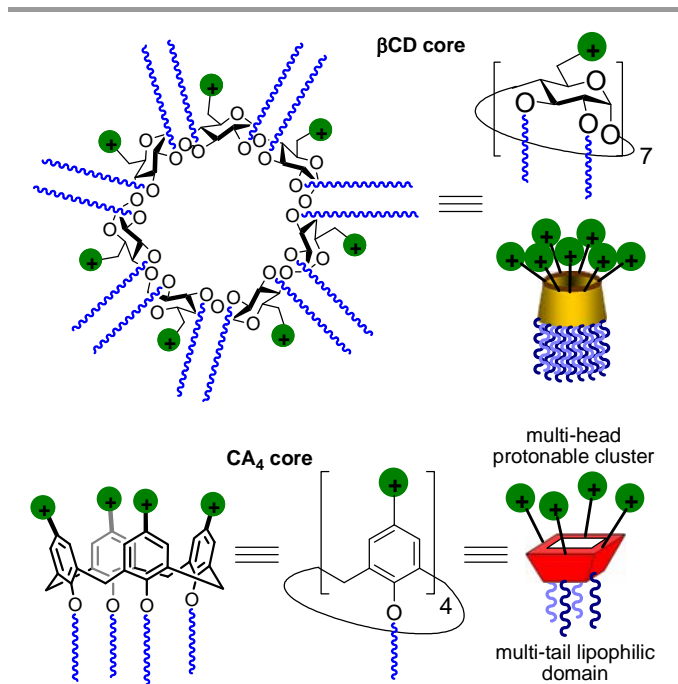
Figure 1. Schematic representation of the amphiphilic polycationic \beta -cyclodextrin ( \beta CD) and calix[4]arene ( CA_4 ) gene vector prototypes in the optimal skirt-type and upper-rim protonable cone arrangements, respectively.
