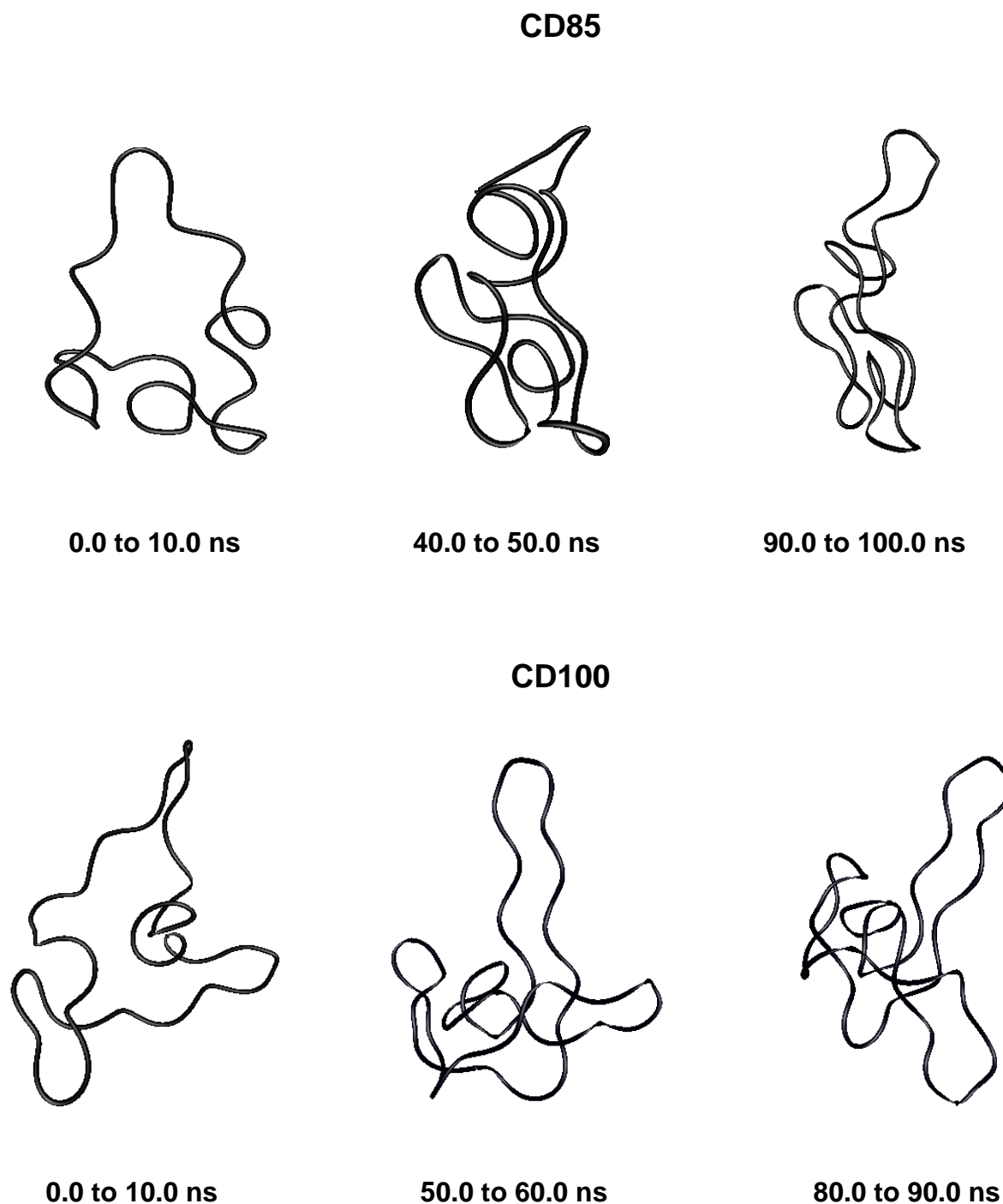
Fig. 3. Averaged structures obtained from analyses of the simulation trajectories of CDn (n=40,70,85,100).
