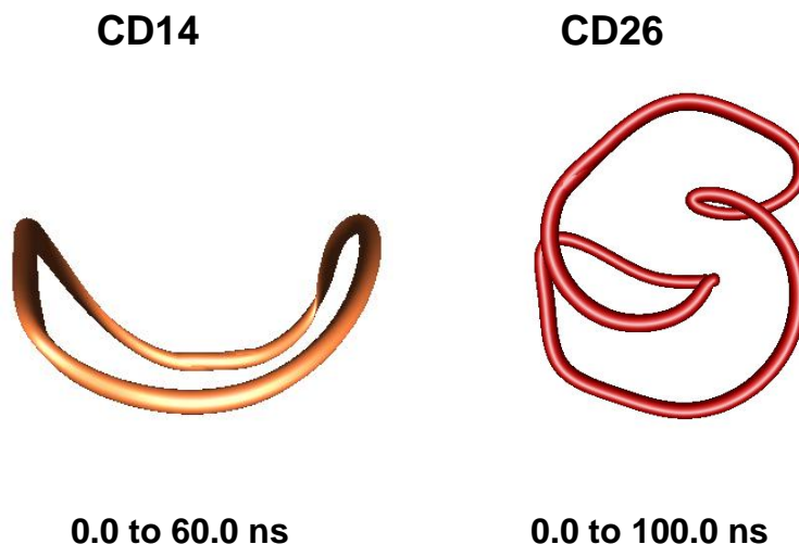
Fig. 2. Averaged structures obtained from analyses of the simulation trajectories of CD14 and CD26.
