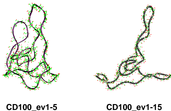
Fig. 5. Characteristic deformations of the macrorings of CDn ( n = 40, 70, 85, 100 ) represented by snapshots (with sequential numbers 1, 5, 10 or 15) of the first animated eigenvectors ( ev1 ).
