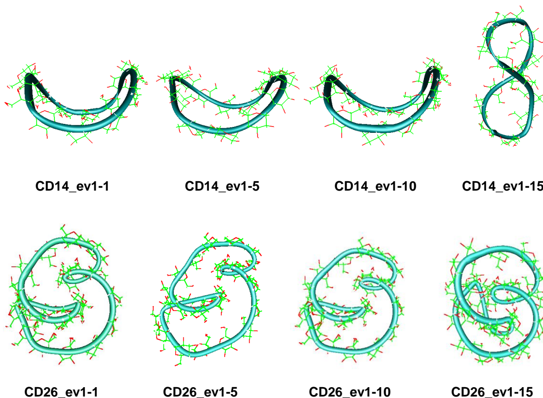
Fig. 4. Snapshots (with sequential numbers 1, 5, 10 and 15) of the first animated eigenvector ( ev1 ) having the largest contribution to the total variance of the atomic fluctuations: (a) CD14 (PCA, 60.0 ns); (b) CD26 (PCA, 100.0 ns).
