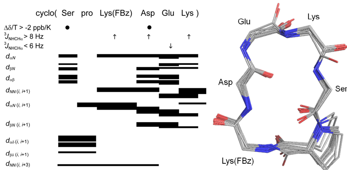
Figure 3. Left: summary of amide NH temperature coefficients ( \Delta\delta/T > -2 ppb/K shown by ●), ^3J_{\text{NHCH}\alpha} coupling constants ( > 8 Hz represented by ↑ and < 6 Hz shown by ↓) and ROEs correlations summary for cyclohexapeptide 3 in DMSO at 298 K. Right: 20-lowest energy structures of 3 . For clarity only the side chain of pro is shown. For summary and structures of cyclohexapeptides 8 and 9 see Supplementary Information (Figure S2). For distance restraints of compounds 3 , 8 and 9 see Tables S1-S3 in Supplementary Information.
