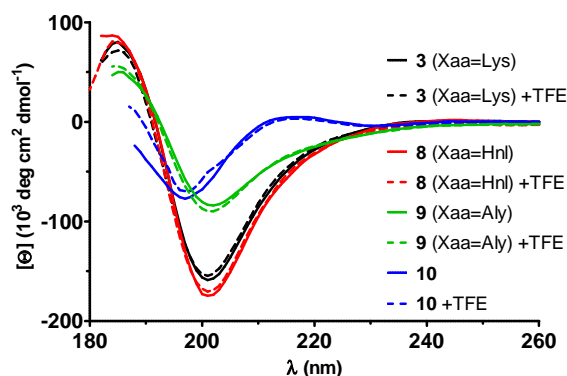
Figure 6. ECD spectra of the cyclohexapeptides 3 , 8 , 9 and the linear analogue 10 in aqueous solution in the absence and presence of trifluoroethanol. The concentration of each peptide was 0.125 mg/mL. The spectra for 0.5 mg/mL can be found in Figure S4 in Supplementary Information.
