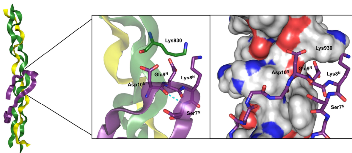
Figure 1. Model of the \alpha 1(I) -N-telopeptide docked to the triple-helical receptor region of bovine type I collagen.
