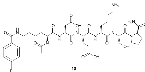
Figure 2. Structure of the linear hexapeptide 10 .
