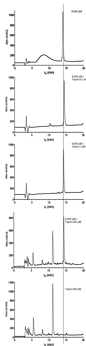
Figure 10. Stability of cyclohexapeptide 3 against cleavage by trypsin as determined by RP-HPLC. Compound 3 was incubated with bovine trypsin at varying concentrations over a time of 30
