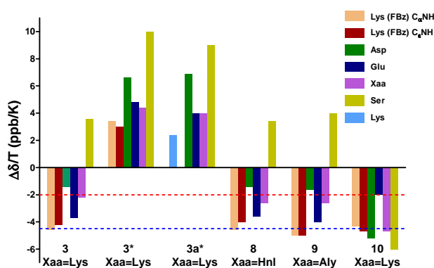
Figure 4. Amide temperature coefficients of the cyclohexapeptides 3 , 3a , 8-9 and the linear hexapeptide 10 in DMSO or water (marked with *).
