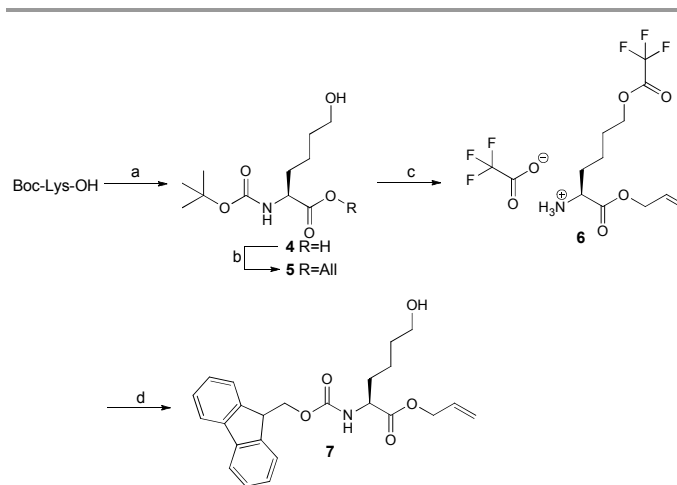
Scheme 3. Synthesis of Fmoc-Hnl-OAll ( 7 ).
