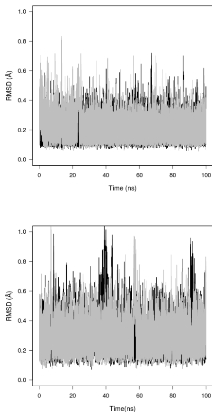
Figure 8. Backbone RMSD of 3 (black) and 9 (grey) in DMSO (top) and water (bottom). Backbone RMSD referred to the mass-weighted least-squares fitting of the average structures after removal of overall translational and rotational motions of 100 ns MD simulations.
