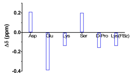
Figure 5. Secondary chemical shifts of C_{\alpha} protons in cyclohexapeptide 3 in aqueous solution referenced to tabulated random coil values ( \Delta\delta = \delta_{\text{CH}\alpha}(\mathbf{3}) - \delta_{\text{CH}\alpha}(\text{random coil}) ). 52
