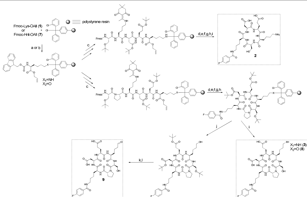
Scheme 2. Synthesis of cyclo(Ser-Lys(FBz)-Asp-Glu-Lys) ( 2 ) and cyclo(Ser-D-Pro-Lys(FBz)-Asp-Glu-Xaa) ( 3 , 8 , 9 ).
