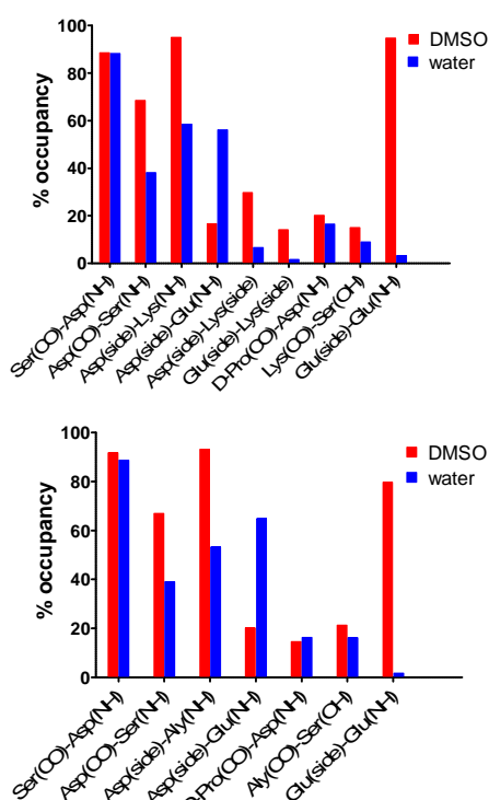
Figure 9. H-bond analysis derived from the 100 ns trajectories in DMSO (red) and water (blue). Top: cyclo(Ser-D-Pro-Lys(FBz)-Asp-Glu-Lys) ( 3 ), Bottom: cyclo(Ser-D-Pro-Lys(FBz)-Asp-Glu-Aly) ( 9 ).
