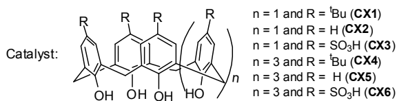
25 Figure 1. Structure of calix[ n ]arenes evaluated as catalyst.
