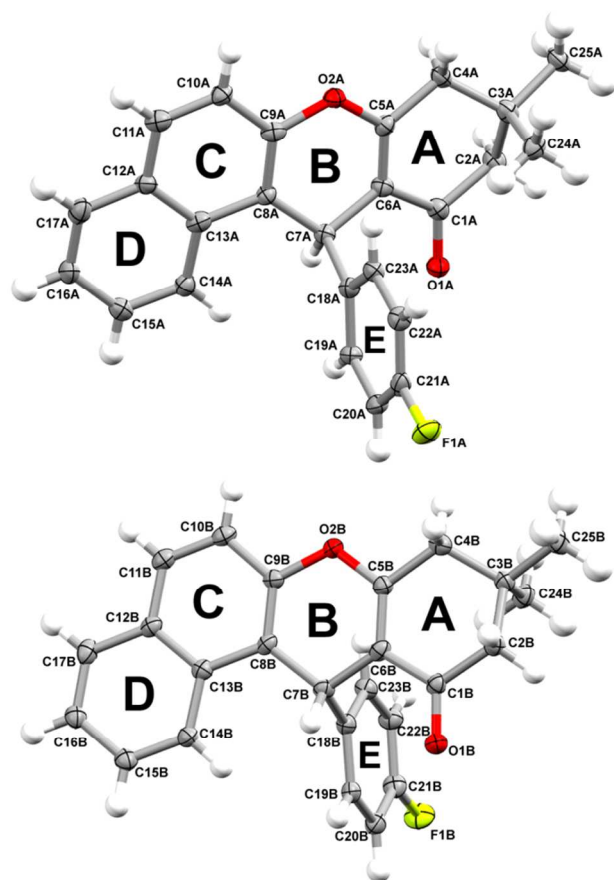
Figure 3. The two crystallographically independent molecules of compound 4 . Ellipsoids of 30% probability and arbitrary radius spheres represent non-hydrogen and hydrogen atoms, respectively. Rings are also arbitrarily labeled.
