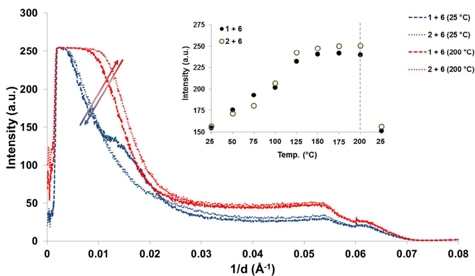
Figure 5. Small angle X-ray scattering from the divalent pyrenyl-polymer blend ([1+6]) and the blend containing the trivalent pyrenyl-polymer ([2+6]). Curves are shown for scattering at 25 °C and 200 °C, and the inset shows the incremental variation in scattering intensity at 1/d = 0.01 \text{ \AA}^{-1} over this temperature range.
