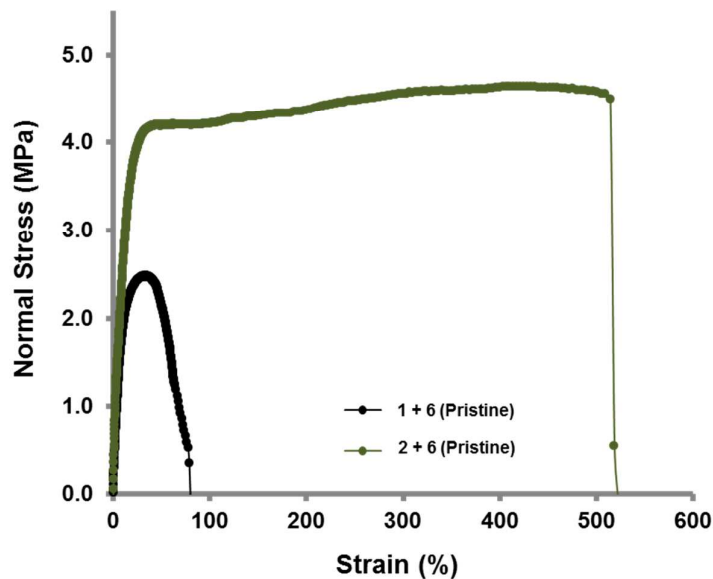
Figure 8. Stress-strain curves for supramolecular polymer blends of polydiimide 6 with the divalent pyrenyl-polymer 1 and trivalent pyrenyl-polymer 2 .
