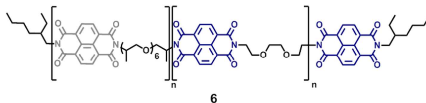
Figure 1. Structure of copolymer 6 , with chain-folding naphthalene-diimide residues (blue) spaced by a linker derived from 2,2'-(ethylenedioxy)bis(ethylamine). The naphthalene-diimide residues (grey) spaced by Jeffamine ® D-400 residues do not form chain-folding sequences.
