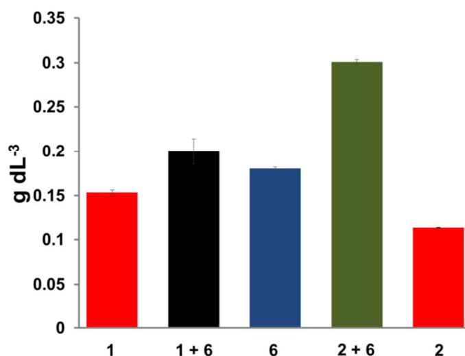
Figure 3. Inherent viscosities of individual polymers ( 1 , 2 and 6 ) and the equimolar (with respect to binding motifs) polymer blends ([ 1 + 6 ] and [ 2 + 6 ]) at 10 mg mL -1 in chloroform/hexafluoroisopropanol (9:1, v/v). Viscosities are the mean of four repeat measurements in each case.
