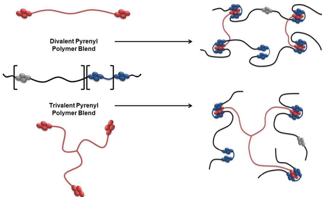
Scheme 2. Schematic for supramolecular polymer blends in which species with different pyrenyl valencies (in red) complex with a chain-folding diimide (blue/black/grey). The naphthalene-diimide residues (grey) spaced by Jeffamine ® D-400 residues do not form chain-folding sequences.
