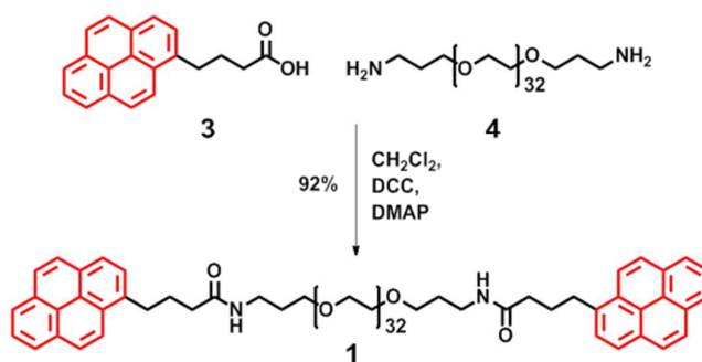
Scheme 3. Synthesis of divalent pyrenyl-terminated poly(ethylene glycol) 1 via DCC coupling. The pyrenyl moieties represent the \pi -electron-rich guests (Scheme 2) which are able to intercalate with a \pi -electron-deficient chain-folding motif.
