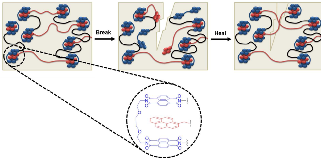
Scheme 1. Schematic of a complementary \pi - \pi stacking polymer blend, illustrating the process of breaking the polymer matrix by disengagement of the weaker supramolecular interactions before applying an appropriate stimulus to facilitate healing. Insert shows the atomistic structure of the \pi - \pi stacked complex 54 with \pi -electron rich pyrenyl end-groups (red) and \pi -electron deficient naphthalenediimide units (blue) linked by an appropriate spacer to form a chain-folding residue.
