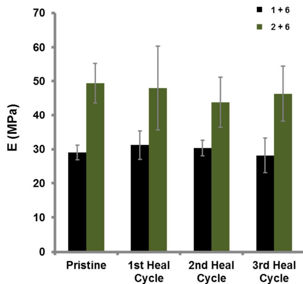
Figure 7. Tensile moduli of the blends containing the divalent pyrenyl-polymer [1+6] and trivalent pyrenyl-polymer [2+6], demonstrating the increased modulus of the pristine blend containing the trivalent pyrenyl polymer (49 MPa) when compared to the pristine divalent pyrenyl polymer blend (29 MPa) as a result of increased supramolecular cross-link density. This difference is maintained over three break/heal cycles.
