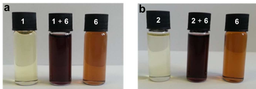
Figure 2. Solutions of the divalent ( 1 ) and trivalent ( 2 ) pyrenyl end-capped polymer in chloroform, and their blends with the chain-folding diimide 6 . The deep red colour of the blends arises from \pi - \pi stacking and charge-transfer between electronically complementary residues.
