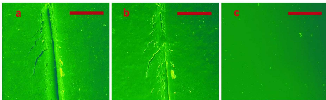
Figure 6. False colour ESEM images of the healable polymer blend [2+6] containing a trivalent pyrenyl-terminated polymer. Micrographs were taken at (a) 25 ^{\circ}\text{C} , (b) 100 ^{\circ}\text{C} and (c) 200 ^{\circ}\text{C} . The images demonstrate both formation of a homogenous blend and the healability of the polymer at elevated temperatures. Scale bar represents 300 \mu\text{m} .
