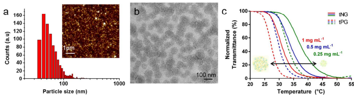
Fig. 2 Characterization of tNGs. (a) AFM statistical analysis of the inserted AFM image (b) TEM image of tNGs (c) Normalized transmittance of tNG solution (solid lines) and corresponding thermoresponsive precursors, tPG (dashed lines), in PBS as a function of temperature at 0.25\text{ mg mL}^{-1} (green), 0.5\text{ mg mL}^{-1} (blue), and 1\text{ mg mL}^{-1} (red).
