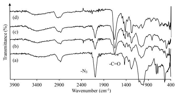
Fig. 5. FT-IR spectra of (a) \text{N}_3\text{-HEC} , (b) \text{HEC-g-PVP}_{10} (1:5 \text{PVP}:-\text{N}_3 ), (c) \text{HEC-g-PVP}_{10} (1:3 \text{PVP}:-\text{N}_3 ), (d) \text{HEC-g-PVP}_{10} (2:1 \text{PVP}:-\text{N}_3 ).
