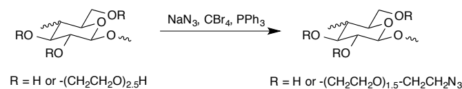
Scheme 1. Synthesis of partially ^{15}\text{N} -labelled \text{N}_3 -HEC
