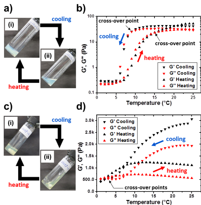
Figure 5. (a) Digital photographs recorded for a 10% w/w aqueous dispersion of (1:9 PCysMA 31 + PGMA 55 )-PHPMA 166 worms recorded at (i) 20 °C (free-flowing liquid) and (ii) 1 °C (free-standing gel). (b) Variation of storage modulus ( G' , black symbols) and loss modulus ( G'' , red symbols) for the same 10% w/w diblock copolymer worm gel during thermal cycling in 1 °C increments: (i) cooling from 25 °C to 1 °C ( G' = inverted black triangles, G'' = inverted red triangles) and (ii) subsequent warming to 25 °C in 1 °C increments ( G' = black triangles, G'' = red triangles). (c) Digital photographs recorded for a 20% w/w aqueous dispersion of (1:9 PGSHMA 24 + PGMA 55 )-PHPMA 178 worms recorded at (i) 20 °C (free-standing gel) and (ii) 1 °C (free-flowing liquid). (d) Variation of storage modulus ( G' , black symbols) and loss modulus ( G'' , red symbols) for the same 20% w/w diblock copolymer worm gel during thermal cycling in 1 °C increments: (i) cooling from 25 °C to 1 °C ( G' = inverted black triangles, G'' = inverted red triangles) and (ii) subsequent warming from 1 °C to 25 °C in 1 °C increments ( G' = black triangles, G'' = red triangles).
