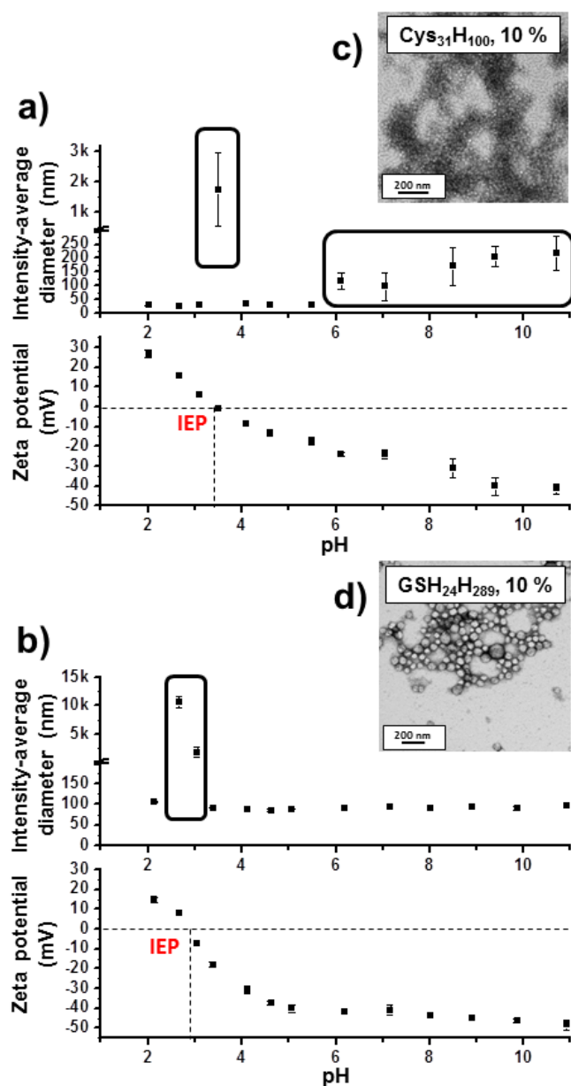
Figure 6. Variation of zeta potential and intensity-average diameter with pH for: (a) PCysMA 31 -PPHMA 100 spheres; and (b) PGSHMA 24 -PPHMA 289 spheres. Each data point was obtained for an individual dispersion diluted to obtain the desired final pH. (c) and (d): Representative TEM micrographs obtained for PCysMA 31 -PPHMA 100 spheres and PGSHMA 24 -PPHMA 289 spheres respectively.
