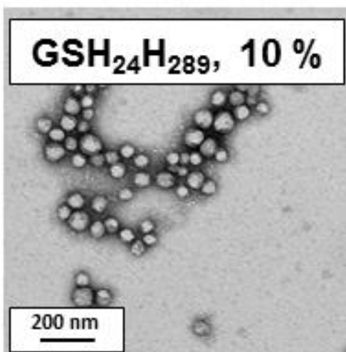
Figure 2. Representative TEM image obtained for PGSHEMA 24 –PPHMA 289 diblock copolymer spheres prepared at 10 % w/w solids via RAFT aqueous dispersion polymerization of HPMA at 70 °C. (PGSHMA and PPHMA are denoted ‘GSH’ and ‘H’ respectively for brevity)
