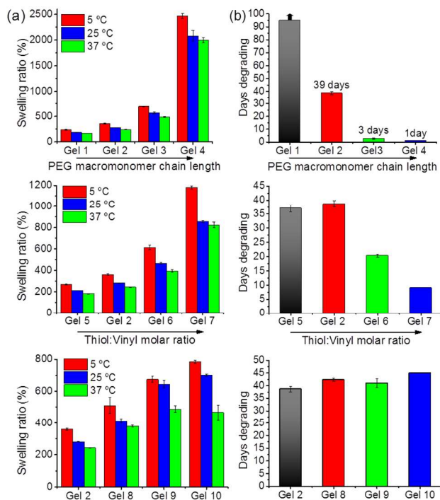
Fig. 2 (a) Deionized water swelling ratios at T = 5 °C (red bars), T = 25 °C (blue bars), and T = 37 °C (green bars) for hydrogels prepared according to Table 1 at increased PEG macromonomer chain lengths (Gels 1-4), increased thiol:vinyl molar ratios (Gels 2, and 5-7), and increased wt% of co-solvent dodecanol used for gel preparation (Gel 2, and Gels 8-10). (b) Time taken to complete degradation of the hydrogels prepared according to Table 1 and shown in the left row immersed in 15 mL 0.1 M PBS at pH = 7.4 and T = 37 °C to mimic physiological conditions.
