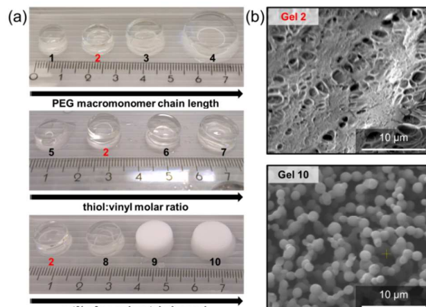
Fig. 1 (a) Photographs of the water-containing hydrogels prepared according to Table 1. All materials were prepared by molding within 4 mL glass vials. Thus, the volume variations observed are due to inherently different water uptake of the gels. (b) Cryo-SEM of Gels 2 and 10.
