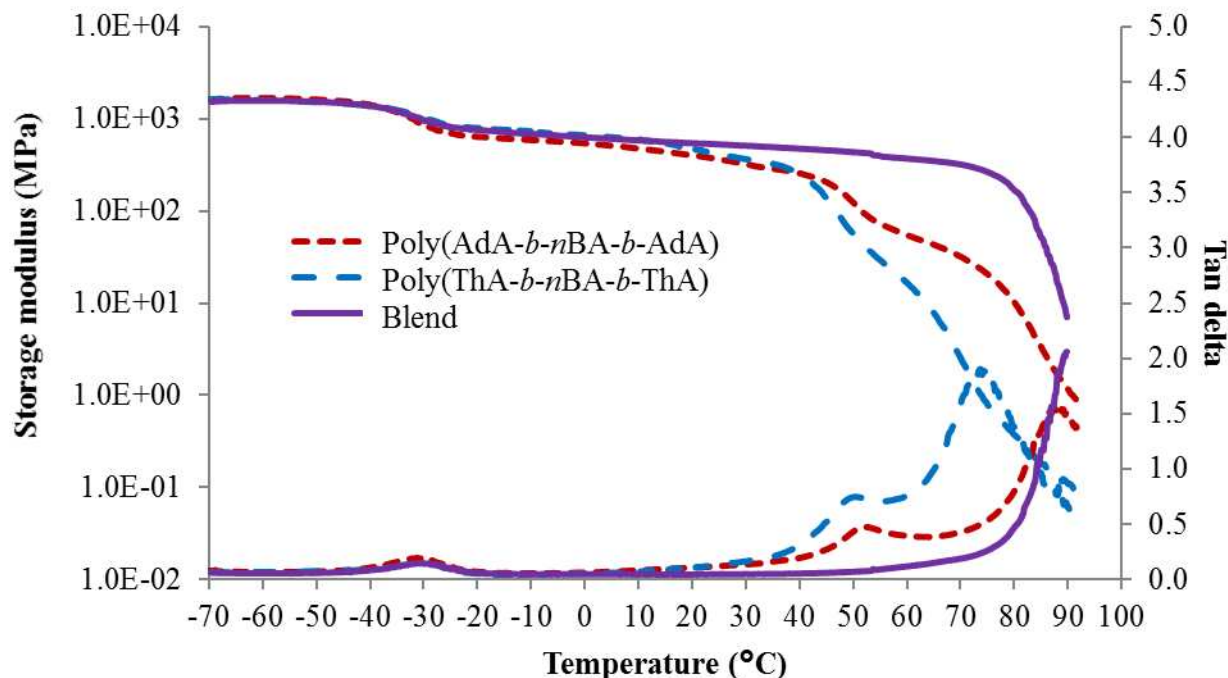
Figure 4. Thermomechanical properties of solution-cast nucleobase-functionalized triblock copolymers and their blend.
