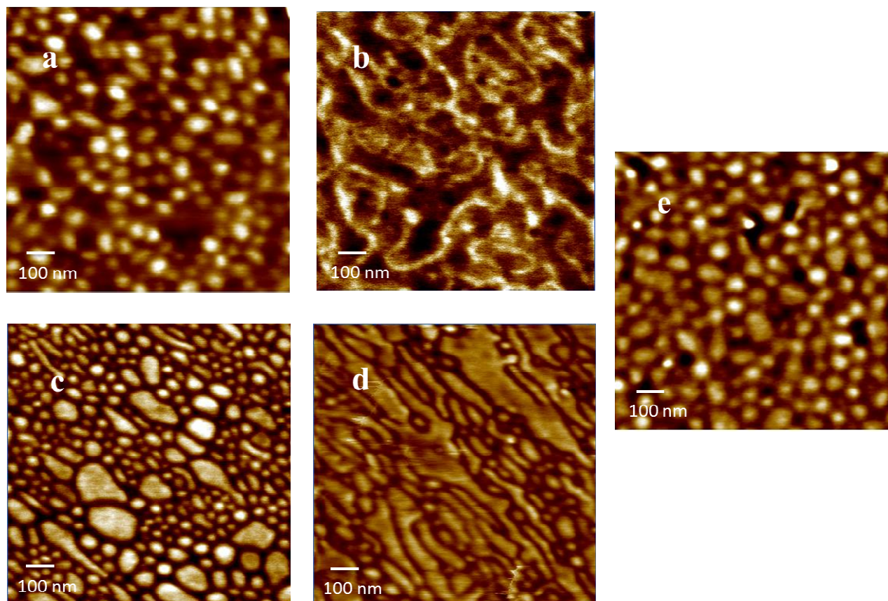
Figure 3. Tapping mode AFM phase image of (a) solution-cast poly(AdA- b - n BA- b -AdA), (b) solution-cast poly(ThA- b - n BA- b -ThA), (c) melt-pressed poly(AdA- b - n BA- b -AdA), (d) melt-pressed poly(ThA- b - n BA- b -ThA), and (e) solution-cast supramolecular blend.
