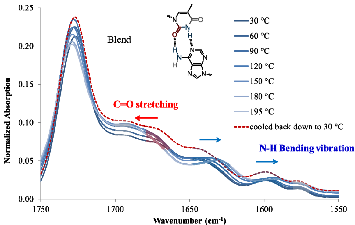
Figure 7. Variable temperature FTIR spectra in the 1500-1700 \text{cm}^{-1} region for the supramolecular blend.
