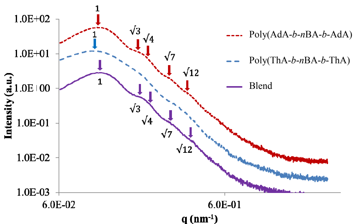
Figure 5. SAXS of solution-cast nucleobase-functionalized triblock copolymers and their blend.
