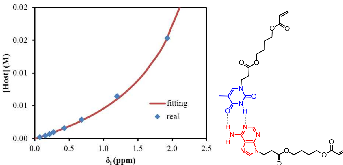
Figure 1. Non-linear fitting of NMR titration results to determine the binding constant of AdA and ThA in \text{CDCl}_3 at 22 \text{ }^\circ\text{C} .
