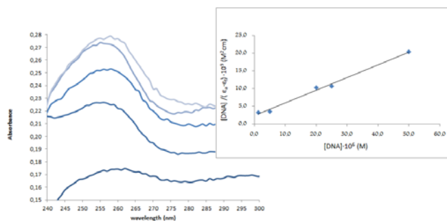
Figure 7. UV absorption spectra of [Pt(\mu-H_3L^1)]_2 in presence of increasing amounts of CT-DNA. Data were collected for [Pt(\mu-H_3L^1)]_2 = 5 \cdot 10^{-6} M and [CT-DNA] = 1.25 \cdot 10^{-6} , 5 \cdot 10^{-6} , 20 \cdot 10^{-6} , 25 \cdot 10^{-6} , 50 \cdot 10^{-6} M. The insert shows a fitting of the absorbance data used to obtain the binding constants.
