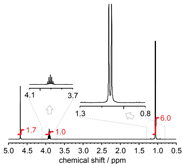
Figure 2. The ^1\text{H} high resolution spectrum of 0.2% (\text{CH}_3)_2\text{CHOH} in \text{D}_2\text{O} .
