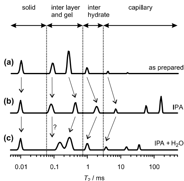
Figure 3. The distribution graph of the T_2 relaxation times for cement paste. The as-prepared sample cured under H_2O , (a); exchanged with isopropanol (b); and exchanged back with H_2O (c).
