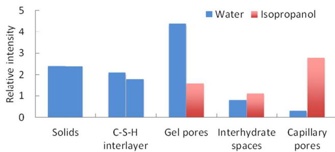
Distribution (by ^1\text{H} NMR intensity) of water and isopropanol in as prepared (left bars) and exchanged (right bars) cement paste.
