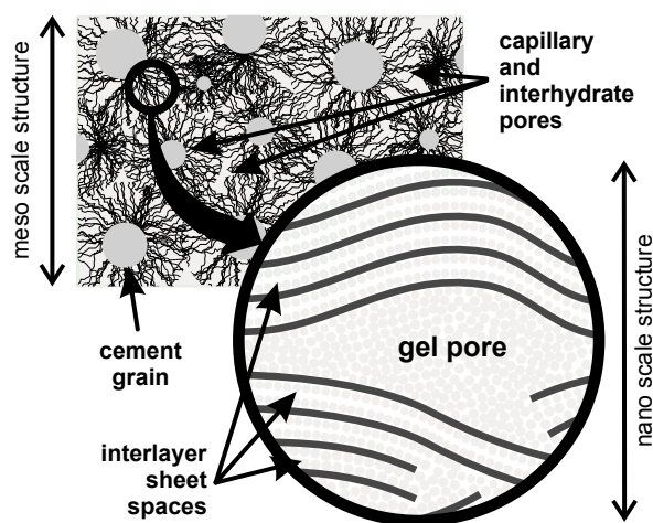
Figure 1. The schematic structure of the calcium-silicate-hydrate (C-S-H) paste on the meso- and nano-scale (white cement paste).
