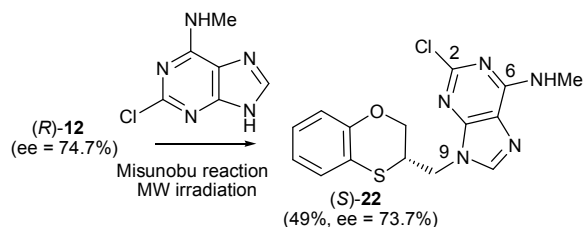
Scheme 10. Preparation of ( S )-( N -9-alkylated-2-chloro- N -methyl)adenine [( S )-22].
