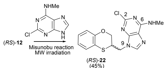
Scheme 8. Preparation of ( RS )-( N -9-alkylated-2-chloro- N -methyl)adenine [( RS )-22].
