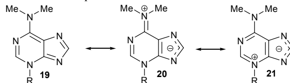
Scheme 7. Resonance hybrid 20 can explain the alkylation at the N -3 atom of the purine moiety, as suggested by non-equivalent -NMe 2 signals in the 1 H NMR spectrum of ( RS )- 17 .
