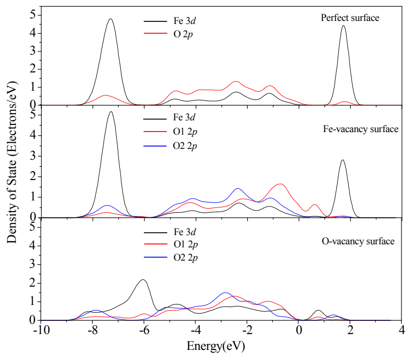
Fig. 4 PDOS for Fe and O atoms on the perfect, Fe-vacancy and O-vacancy \alpha\text{-Fe}_2\text{O}_3(0001) surfaces
