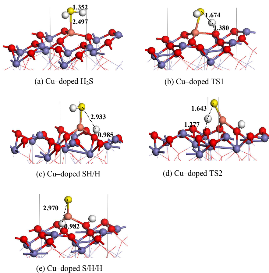
Fig. 7 The reactant, intermediate and transition state structures in the dissociation of H 2 S on the Cu-doped surface.
