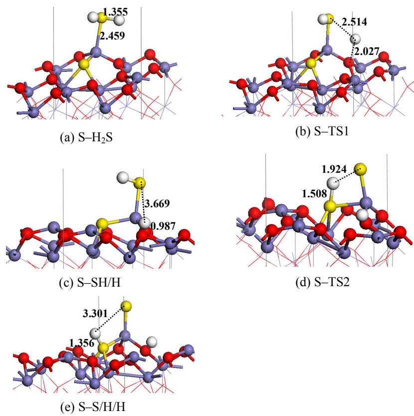
Fig. 6 The reactant, intermediate and transition state structures for the dissociation of H 2 S on the sulfurized surface.
