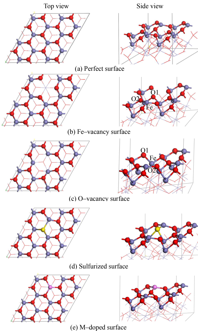
Fig. 2 The optimized structures of different \alpha\text{-Fe}_2\text{O}_3(0001) surfaces, top and side views (a) Perfect surface (b) Fe–vacancy surface (c) O–vacancy surface (d) Sulfurized surface (e) M–doped surface. Purple, red, yellow and pink balls are represented Fe, O and S and the substituted metal atoms, respectively.
