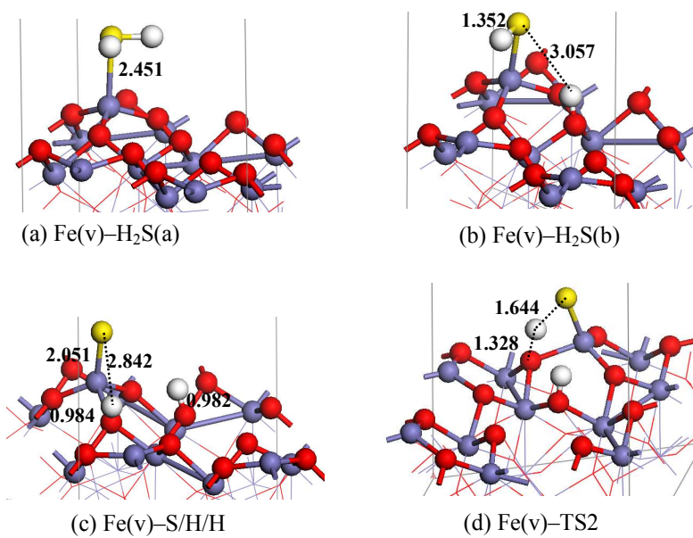
Fig. 5 the optimized structures of H 2 S and its dissociation species adsorption on the Fe-vacancy surface as well as transition states of dissociation.
