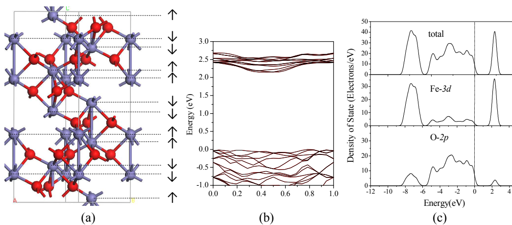
Fig. 1 The structure and electronic properties of \alpha -Fe 2 O 3 . (a) The hexagonal crystal structure of antiferromagnetic \alpha -Fe 2 O 3 and the spin arrangements; (b) calculated electronic band structure; (c) total and PDOS analysis of antiferromagnetic \alpha -Fe 2 O 3 .
