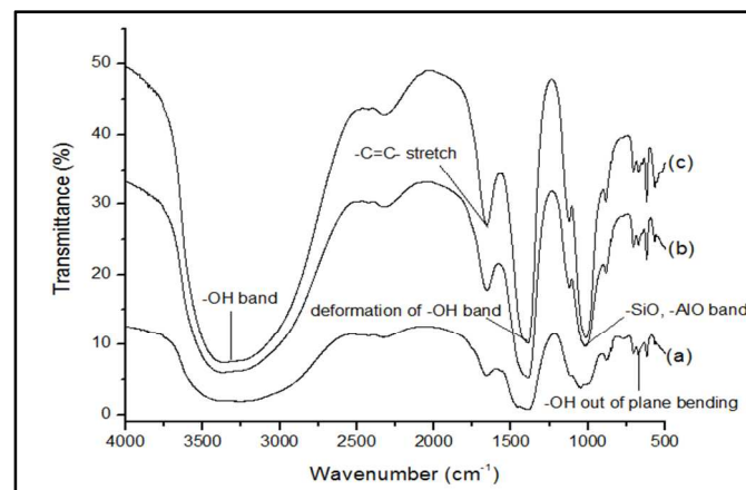
Figure 9: FTIR spectra of a) BA 110, b) BA 700 and c) BA 900.
