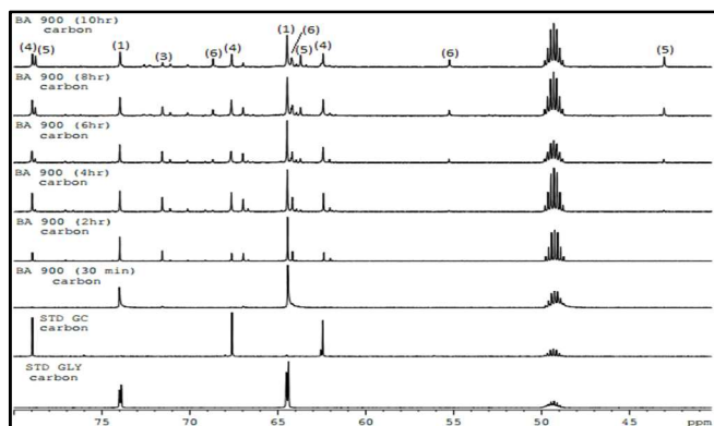
Figure 6(a): 13 C NMR overlay of standard glycerol (STD GLY), standard glycerol carbonate (STD GC) and TOL of BA 900. Key: (1) Glycerol; (3) 2, 3-dihydroxypropyl carbamate, (4) Glycerol carbonate; (5) 4-(hydroxymethyl) oxazolin-2-one; (6) (2-oxo-1,3-dioxolan-4-yl) methyl carbamate.
