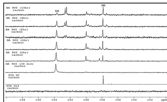
Figure 6(b): 13 C NMR overlay of standard glycerol (STD GLY), standard glycerol carbonate (STD GC) and TOL of BA 900. Key: (2) Urea and (4) Glycerol carbonate.
