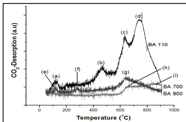
Figure 12: \text{CO}_2 -TPD of BA 110, BA 700 and BA 900.
