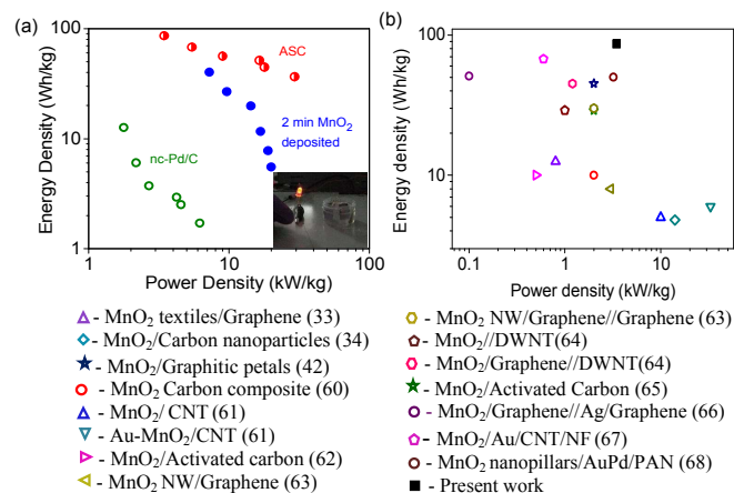
Fig. 6 Ragone plots for the nc-Pd/C, MnO 2 /nc-Pd/C and MnO 2 /nc-Pd/C//nc-Pd/C ASC in 1M Na 2 SO 4 . Inset shows the glowing red LED after connecting to the three cells in series. (b) Ragone plot comparing a ASC from this study with various MnO 2 coated carbon based supercapacitors from the literature.
