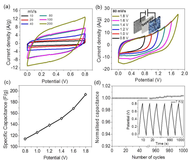
Fig 5 (a) CV curves of (2 minutes) MnO 2 /nc-Pd/C//nc-Pd/C asymmetric supercapacitor (ASC) measured at different scan rates between 0 and 0.8 V. (b) CV curves of the ASC measured at different potential windows at a scan rate of 80 mV/s. (c) Specific capacitances of the ASC obtained for increasing potential window at a scan rate of 80 mV/s. (d) Cycling stability of the ASC over 1000 cycles of charge-discharge cycles at a current density of 7 A/g. Inset shows the charge-discharge curves of the device.
