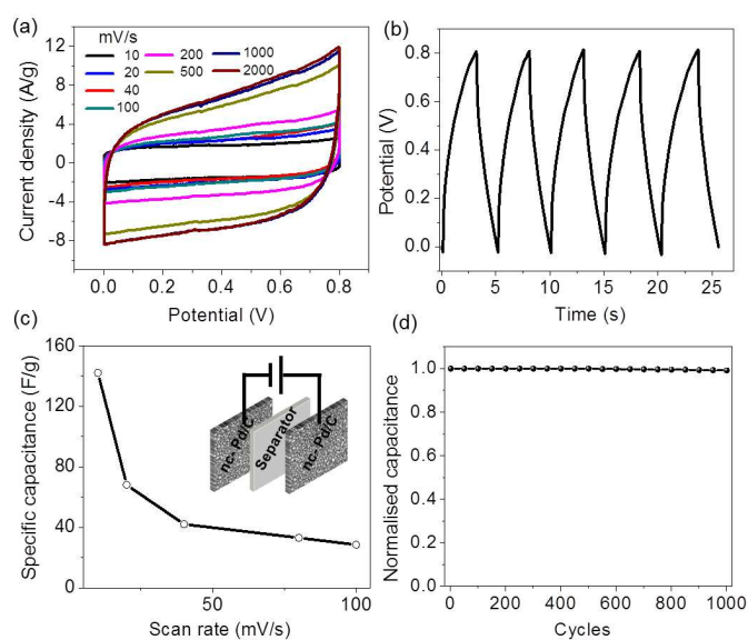
Fig. 2 The performance of the symmetric nc-Pd/C electrochemical capacitor in aqueous 1M Na 2 SO 4 solution. (a) Cyclic voltammograms (CV) at different scan rates, from 10 to 2000 mV/s. (b) Galvanostatic charge/discharge (CD) curves at a current density of 5 A/g. (c) Specific capacitance as a function of scan rate, inset shows the two-electrode configuration of the symmetric nc-Pd/C electrodes along with the separator. (d) Normalized capacitance vs. number of cycles showing the electrochemical stability of nc-Pd/C electrodes over 1000 cycles (data points corresponding to every 50 th cycle, are shown).
