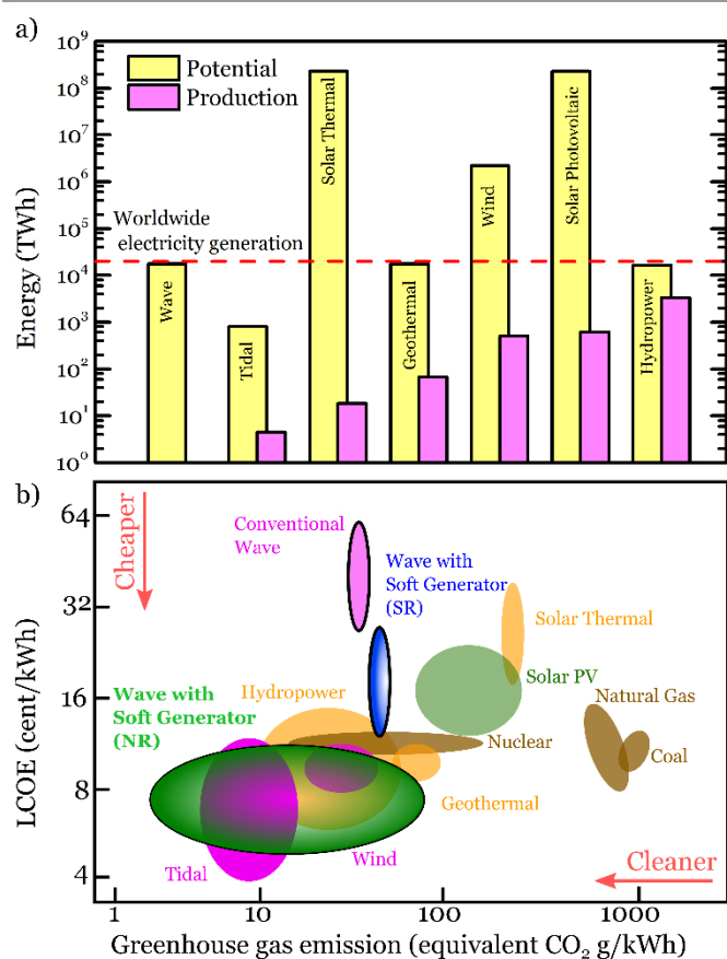
Figure 7 | Natural rubber-based soft generators as a clean and economical method to convert mechanical energy of ocean waves to electricity. a) The full potential of major sources of renewable energy (yellow bars) and their actual contribution to electricity production (pink bars). The full potential of wave energy is on par with the worldwide electricity generation, and is comparable with hydropower and geothermal sources; but its annual production is negligible. Wave energy therefore presents a huge untapped source of clean energy. b) Production cost (LCOE) versus carbon footprint (Greenhouse gas emission) of various energy sources (both renewable and fossil fuel). Harvesting energy from ocean waves with existing technologies (conventional wave) emits twenty times less greenhouse gas than natural gas and coal, but its levelized cost of electricity (LCOE) is more than four times higher. High LCOE prevents large scale exploitation of wave energy. Soft generators based on silicone rubber (in blue) already halve the level of LCOE compared to conventional techniques. On the other hand, natural rubber-based soft generators (in green) can significantly reduce LCOE and greenhouse gas emission.
