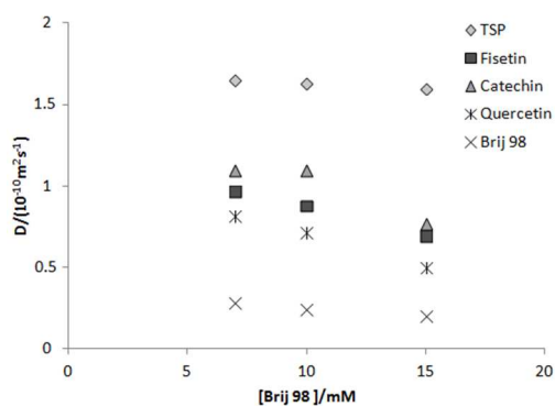
Figure 5 Diffusion coefficients as a function of Brij 98 concentration for a 50% v/v DMSO- d_6 /D _2 O solution containing with trimethylsilyl propionate (TSP) as reference and 5.0 mM of each flavonoid.
