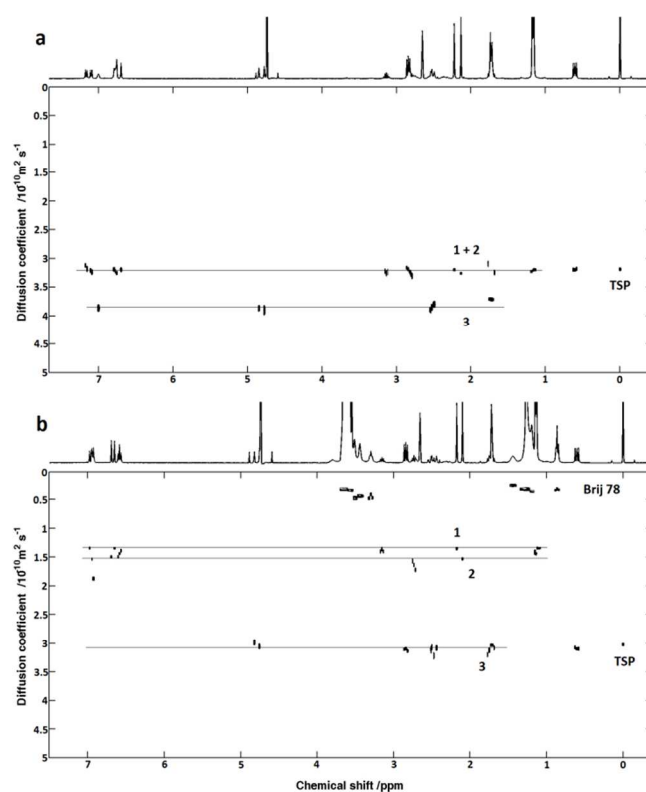
Figure 2 Oneshot DOSY spectra of monoterpenes 1, 2 and 3, in 20% DMSO-d 6 /80% D 2 O (v/v) before (a) and after (b) addition of 5 mM Brij 78.
