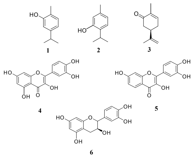
Scheme 2 Structures of the monoterpenes carvacrol (1), thymol (2) and L(-)-carvone (3) and flavonoids quercetin (4), fisetin (5) and (+)-catechin (6).
