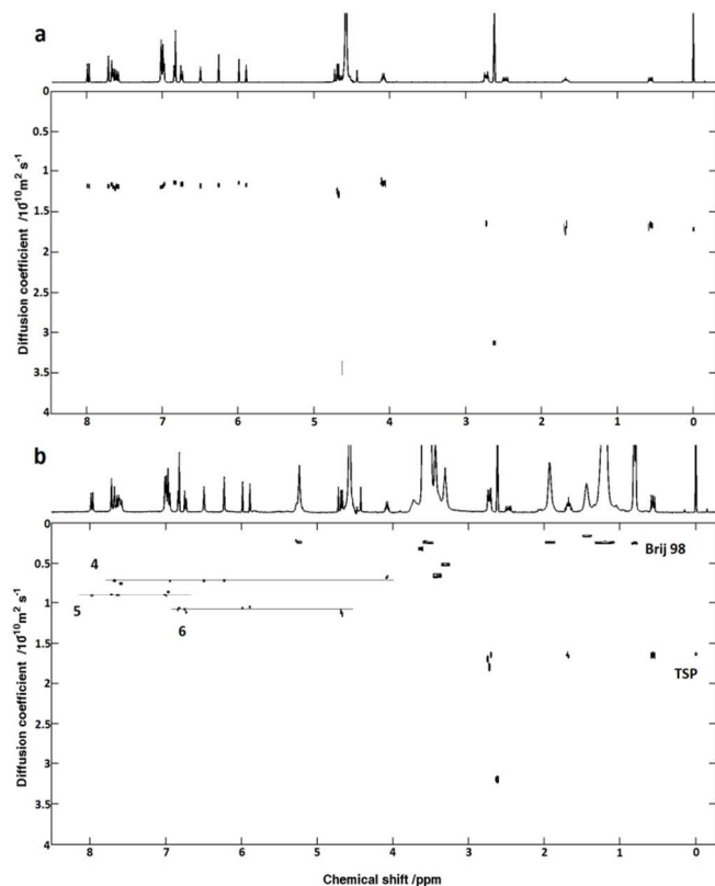
Figure 4 Oneshot DOSY spectra of flavonoids 4, 5 and 6, before (a) and after (b) addition of Brij 98 (10 mM) in 50% v/v DMSO- d_6 /D _2 O. Contour levels are set to show a representative proportion of reporter signals.
