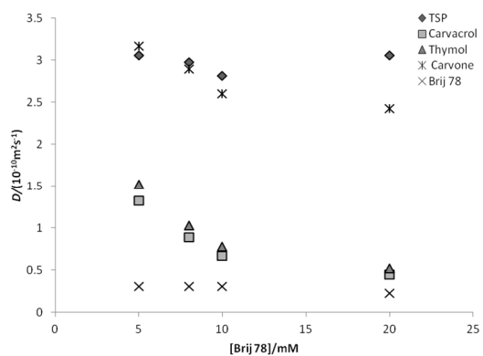
Figure 3 Diffusion coefficients as a function of Brij 78 concentration for a 20% DMSO-d 6 /80% D 2 O (v/v) solution containing trimethylsilyl propionate (TSP) as reference and 3.0 mM of each of monoterpenes 1, 2 and 3.
