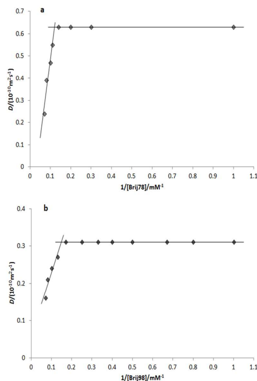
Figure 1 Plot of measured diffusion coefficient, D , against inverse of total surfactant concentration (a) for Brij 78 in 20% DMSO-d 6 /80% D 2 O (v/v) (b) for Brij 98 in 50% DMSO-d 6 /50% D 2 O (v/v).
