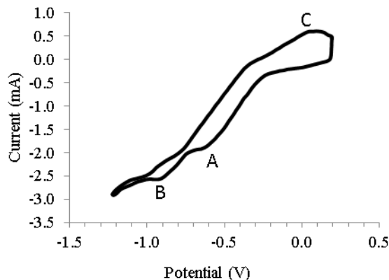
Figure 1- Cyclic voltammogram obtained at a gold working electrode using a NaCl-KCl melt (molar ratio of 1:1) at a temperature of 750 °C under a carbon dioxide pressure of 1.0 MPa. Counter electrode: glassy carbon or platinum crucible; reference electrode: platinum quasi-reference electrode; scan rate: 0.1 V s -1 . (This figure is re-plotted from Ref. 24.)
