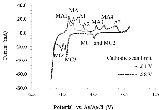
Figure 3 - Cyclic voltammograms obtained using a stainless steel wire working electrode in a molten \text{Li}_2\text{CO}_3\text{-Na}_2\text{CO}_3 electrolyte (molar ratio of 52:48) at 627^\circ\text{C} , at a scan rate of 100\text{ mV s}^{-1} , for negative potential limits of -1.81\text{ V} and -1.88\text{ V} . Atmosphere: \text{CO}_2 ; WE diameter: 0.25\text{ mm} ; WE immersion depth: ca. 1.5\text{ cm} ; CE: 6\text{ mm} diameter stainless steel rod; RE: alumina membrane \text{Ag/AgCl} .
