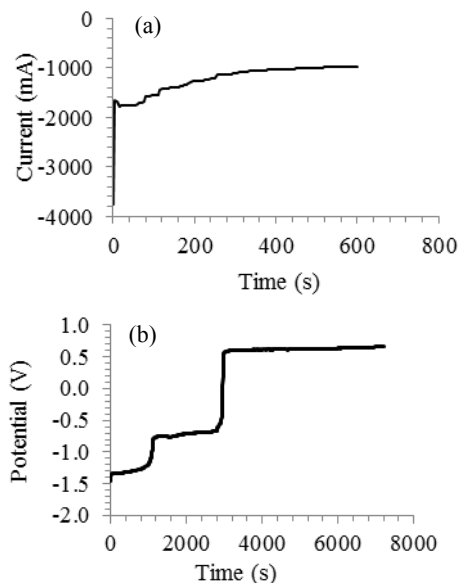
Figure 6– (a) Current-time plot recorded at -2.77 V vs. Ag/AgCl during electrolysis in a molten \text{Li}_2\text{CO}_3\text{-Na}_2\text{CO}_3 (mole ratio: 62:38) at 600 °C on a 5 mm diameter mild steel working electrode; Counter electrode: 6 mm diameter stainless steel rod; Reference electrode (RE): Alumina membrane Ag/AgCl. (b) Potential-time plot recorded during the re-oxidation of carbon deposited in (a); Constant current applied: 150 mA; Temperature: 600 °C; WE: 5 mm diameter mild steel rod (with carbon deposit still attached); CE: 10 mm diameter graphite rod; alumina membrane Ag/AgCl RE.
