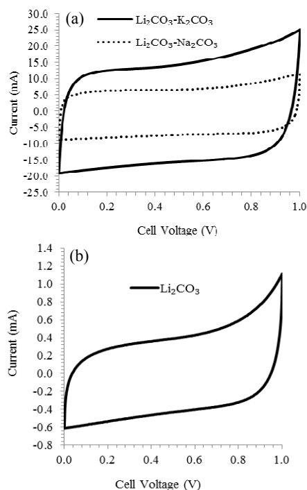
Figure 5 - CVs of symmetrical unit cells constructed with carbon deposited at a cell voltage of 4 V under \text{CO}_2 in (a) \text{Li}_2\text{CO}_3\text{-K}_2\text{CO}_3 (62:38 mol %) at 600 °C and \text{Li}_2\text{CO}_3\text{-Na}_2\text{CO}_3 (52:48) 632 °C (b) \text{Li}_2\text{CO}_3 ; Scan rate: 10 \text{mV s}^{-1} ; Mass of each electrode: 30 mg; Electrolyte : 3 mol \text{L}^{-1} \text{KCl} ; Current collector: titanium foil . The carbon material combined with 5 wt. % Polytetrafluoroethylene (PTFE) was pressed into 13 mm diameter pellets (0.34 mm thick).
