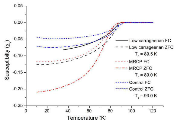
Figure 5. SQUID magnetometry of the control sample, and samples prepared using low ratios of \kappa -carrageenan and MRCP.
