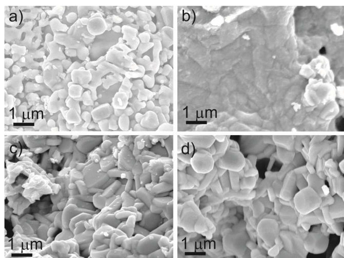
Figure 3. SEM micrographs showing the morphologies found using different templates. a) High ratio \kappa -carrageenan sample with similar reticulated blocky structure to b) low-ratio of \kappa -carrageenan sample. c) Crystallographically and morphologically inhomogeneous control sample. d) The sample templated using MRCP with similar structure to the \kappa -carrageenan samples.
