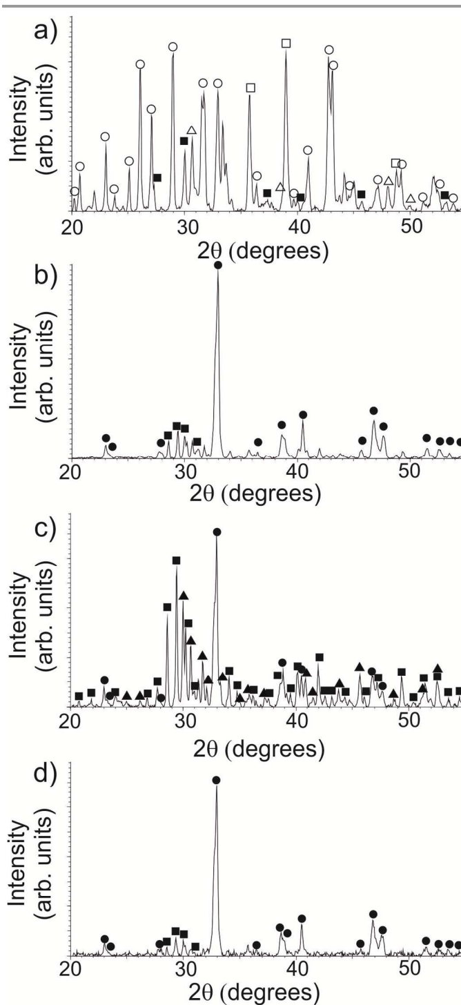
Figure 1. PXRD of the different samples: a) high-ratio \kappa -carrageenan; b) low-ratio \kappa -carrageenan; c) control sample containing no template; and d) MRCP-templated sample. Phases are marked as Y123 (●), BaCuO 2 (■), BaSO 4 (○), Y 2 O 2 S (Δ), CuO (□), and Y211 (▲).
