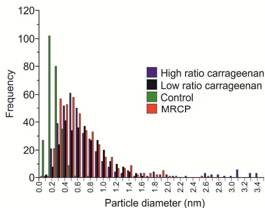
Figure 4. Histogram plots of crystallite size, measured using the longest dimension of the crystallites
