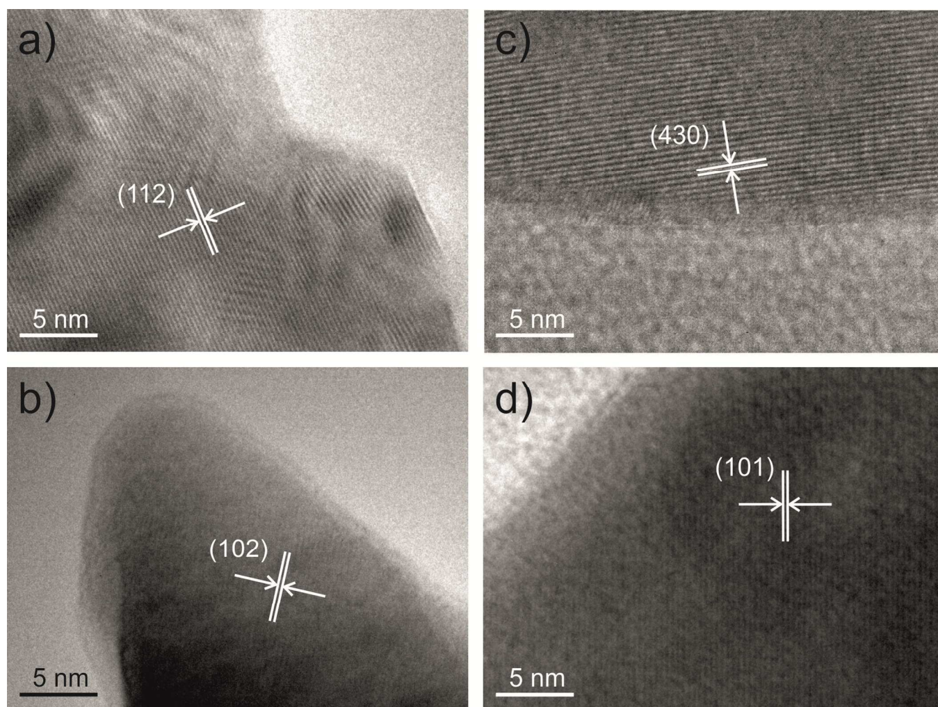
Figure 2. TEM micrographs of the major phase in each sample. a) the high-ratio sample with BaSO 4 lattice planes highlighted; b) the low-ratio sample with Y123 lattice planes highlighted; c) the control sample with BaCuO 2 lattice planes highlighted; and d) the MRCP-templated sample with Y123 lattice planes highlighted.
