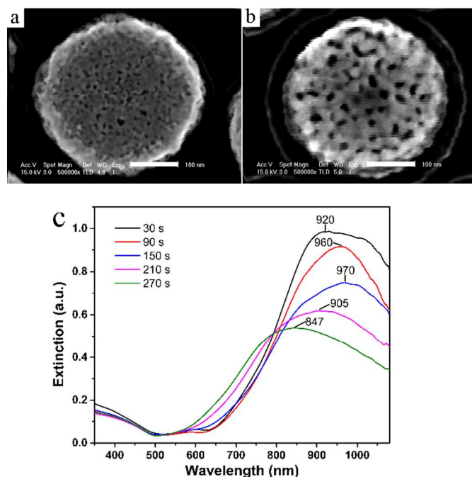
Figure 3 SEM images and extinction spectra of ~300 nm diameter NPG disk made from \text{Ag}_{70}\text{Au}_{30} alloy: (a) and (b) are the SEM images of NPG disk at 30s and 270 s, and (c) extinction spectra versus dealloying time. SEM scale bar: 100 nm.
