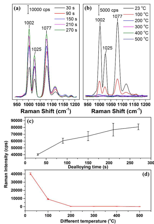
Figure 7 Surface-enhanced Raman spectra of benzenethiol ranging from 930 to 1210 cm -1 on NPG nanoparticles obtained from Ag 82.5 Au 17.5 alloy: (a) different dealloying time and (b) different annealing temperatures for NPG nanoparticles obtained after 30 s dealloying; (c) and (d) are the change trends of intensity of the SERS band at 1077 cm -1 corresponding to different dealloying time and temperatures, respectively.
