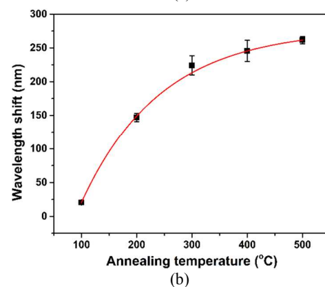
Figure 5 Extinction spectra of 300 nm as-dealloyed NPG nanoparticles from \text{Ag}_{82.5}\text{Au}_{17.5} alloy at 30 s before and after annealing: (a) extinction bands after annealing at different temperatures and (b) the wavelength blue shift as a function of annealing temperatures.
