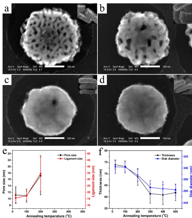
Figure 4 SEM images of NPG nanoparticles after different annealing temperature: (a) 100, (b) 200, (c) 300, and (d) 400 °C. The insets show thickness. (e) the changes of pore and ligament size versus annealing temperature, and (f) is the thickness and NPG disk diameter versus annealing temperature. SEM scale bar: 100 nm.
