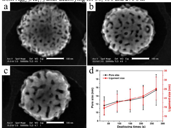
Figure 1 SEM images and image analysis of 300 nm diameter NPG nanoparticles made from Ag 82.5 Au 17.5 alloy for different dealloying time: (a) 30, (b) 150 and (c) 270 s. (d) pore and ligament sizes based on statistical analysis versus dealloying time. SEM scale bar: 100 nm.
