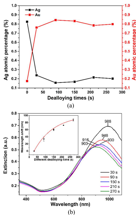
Figure 2 Elemental composition and extinction spectra of 300 nm diameter NPG disk made from Ag 82.5 Au 17.5 alloy: (a) atomic percentage of Ag and Au versus dealloying time. (b) extinction spectra versus dealloying time. The inset shows blueshift versus dealloying time. The curve is only for visual guidance.
