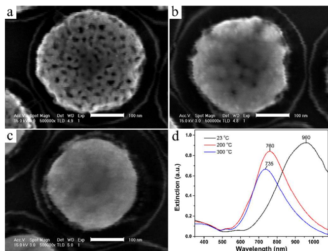
Figure 6 SEM images of ~300 nm NPG nanoparticles dealloyed at 90 s from \text{Ag}_{70}\text{Au}_{30} alloy at (a) 23 °C, (b) 200 °C and (c) 300 °C. (d) Extinction spectra at corresponding temperatures. SEM scale bar: 100 nm.
