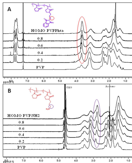
Fig. 3: (A) 1 H-NMR spectra of poly (VP-co-VPPhta) copolymers and homopolymers in CDCl 3 and (B) poly (VP-co-VPNH 2 ) copolymers and homopolymers in D 2 O. PVP spectra have been included for comparative purposes.
