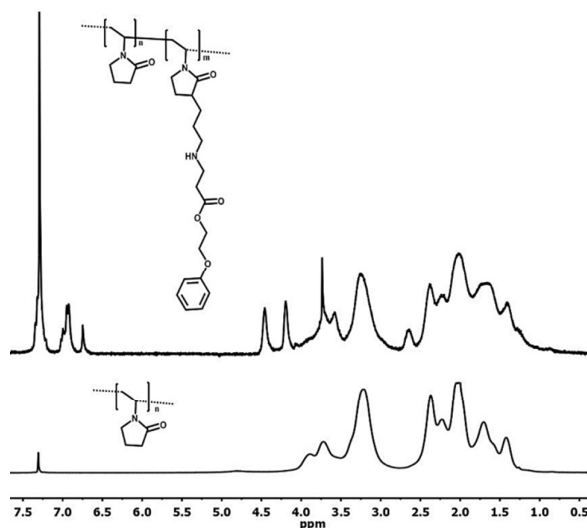
Fig. 6: ^1\text{H} -NMR spectrum of the conjugate Poly VP-2PE 20 , recorded in \text{CDCl}_3 . The spectrum of PVP has been included for comparative purposes.
