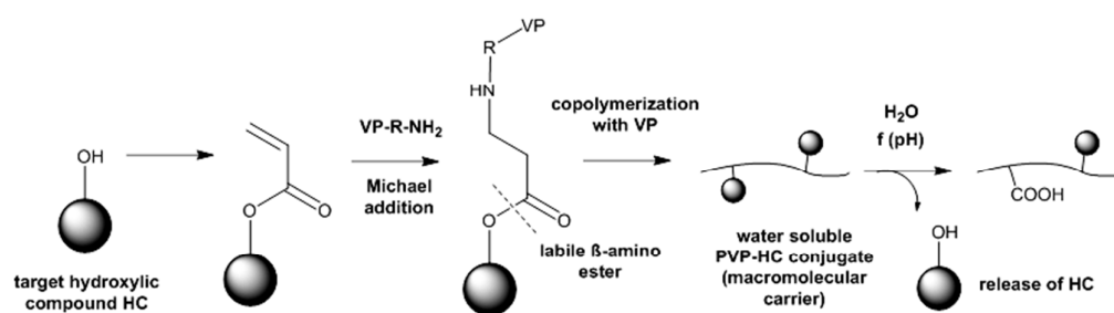
Fig. 4: Synthetic route designed in this work to prepare hydrolysable conjugates of PVP with hydroxyl group-containing drugs from the aminated VP.
