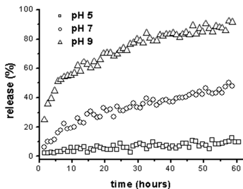
Fig. 8: Release percentage, R, versus time at different pHs obtained by in situ ^1\text{H-NMR} monitoring as explained in the text.
