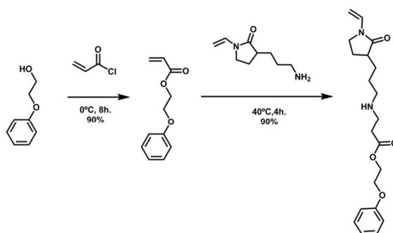
Fig. 5: Synthetic scheme of the VP-2PE conjugate.
