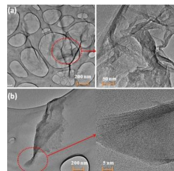
Fig. 3: TEM images of (a) pristine GO and (b) GO functionalized with choline formate.
