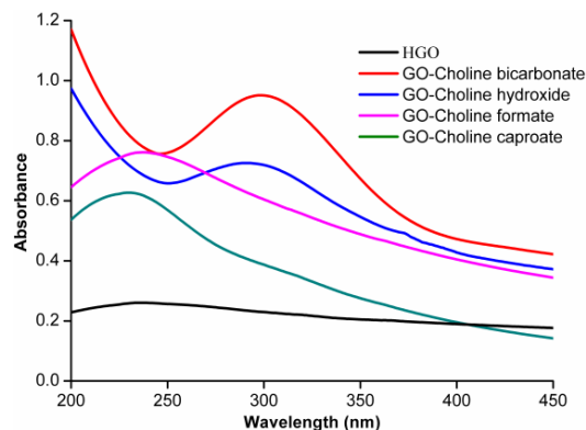
Fig. 2: UV-Vis spectra of pristine GO and IL functionalized GO measured a dilution (50 \mu\text{g}/\text{ml} )
