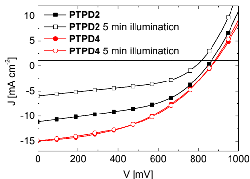
Figure 6. J-V -characteristics for devices using PTPD2 (squares) and PTPD4 (circles) as HTL. Both HTLs are doped and contain the additives LiTFSI and TBP. The filled symbols represent the first measurement, the unfilled symbols the measurement after five minutes illumination under light. All devices were measured at a simulated AM1.5G solar irradiation of 100 \text{ mW cm}^{-2} under ambient conditions.
