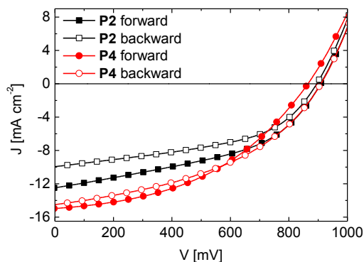
Figure 5. J-V -characteristics for devices using PTPD2 (squares) and PTPD4 (circles) as HTL, both doped and with LiTFSI and TBP as additives. The forward scan (filled symbols) and backward scans (empty symbols) were measured at a simulated AM1.5G solar irradiation of 100 \text{ mW cm}^{-2} under ambient conditions.
