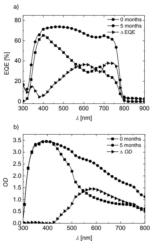
Figure 8. Comparison of devices with PTPD2 doped and containing LiTFSI and TBP as additives: freshly prepared (squares), stored devices, and difference of both (triangles). a) EQE-spectra; The artifact between 650–700 nm is due to the switching of the lamp from one wavelength range to the other. b) UV-vis absorption. All measurements were carried out under ambient conditions.
