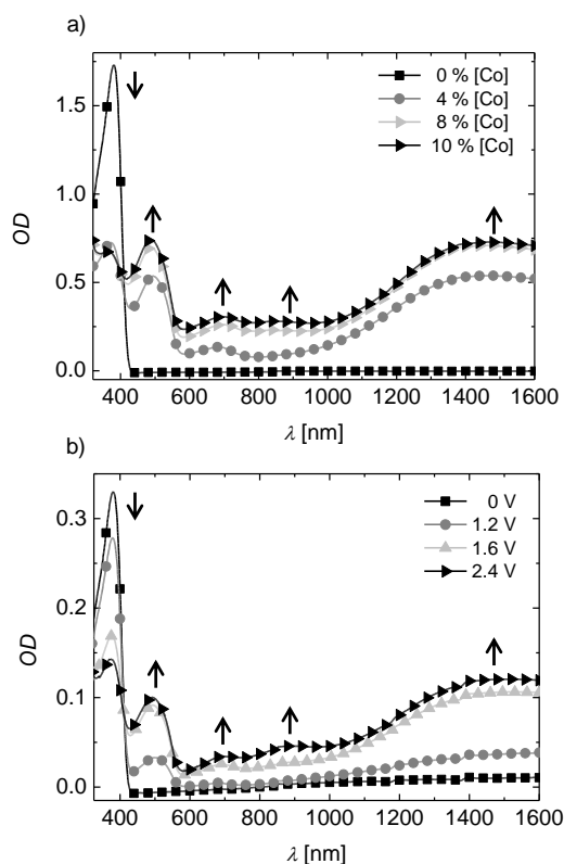
Figure 2. a) UV-vis-NIR absorption spectra of PTPD2 in THF solution ( 0.025 \text{ mg ml}^{-1} ). Stepwise addition of the Co(III)-complex leads to four new bands at 490, 694, 860 nm, and 1403 nm. b) Spectroelectrochemical measurements in THF with 0.1 M tetrabutylammonium hexafluorophosphate as conducting salt resemble the oxidative doping.
