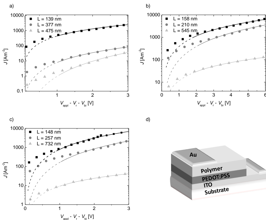
Figure 1. Log-linear plots of current density J vs. voltage V (data points) and fits according to equation 1 (straight lines) at room temperature for the hydrophobic polymers a) PTPD2 and b) PTPD3 as well as for the hydrophilic polymer c) PTPD4 for different layer thicknesses; d) Scheme of a hole only device with gold as top electrode and PEDOT:PSS as bottom electrode.
