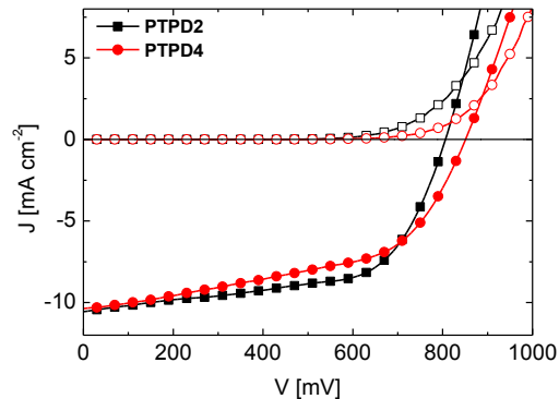
Figure 4. J - V -characteristics in light (filled symbols) and in dark (empty symbols) for the best devices with PTPD2 (squares) and PTPD4 (circles) both doped and containing the additives LiTFSI and TBP. The devices were measured in air immediately after preparation at a simulated AM1.5G solar irradiation of 100 mW cm -2 in forward bias.
