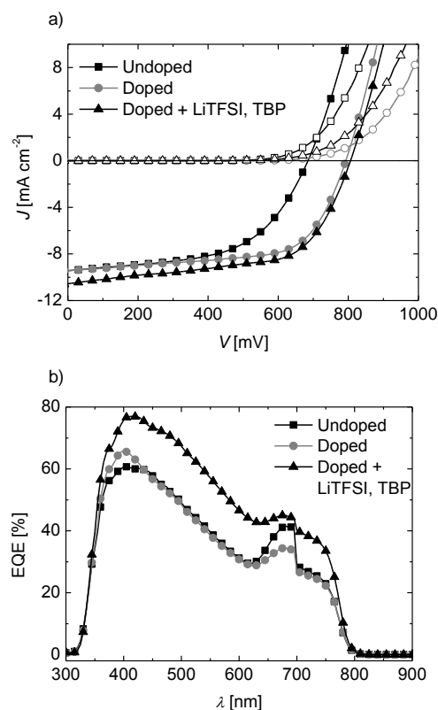
Figure 3. Photovoltaic characterization of devices using PTPD2 undoped (squares), doped (circles), and doped containing the additives LiTFSI and TBP (triangles) measured immediately after preparation. a) J - V -characteristics of the three photovoltaic devices (best cells) measured at a simulated AM1.5G solar irradiation of 100 \text{ mW cm}^{-2} in forward bias under ambient conditions. b) EQE-spectra of the devices measured under ambient conditions. The artifact at about 700 nm is due to the switching of the lamp from one wavelength range to the other.
