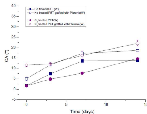
Fig. 8 Contact angle of modified PET versus immersion time in water.
