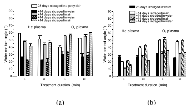
Fig. 5 Contact angle of PET films treated with (a) He and (b) O 2 plasmas after switching the storage conditions (water or air).
