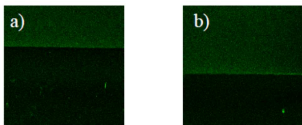
Fig. 9 confocal microscopy image of oboalbumin adsorption by biorecognition assay onto a PET surface where the lower part of the sample is treated with (a) He and (b) O 2 plasma (scale : 158 x 158 μm).
