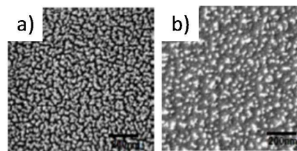
Fig. 3. SEM images of surfaces treated for 30 min with He plasma (a) and with O 2 plasma.
