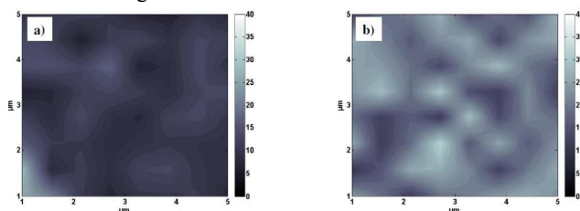
Fig. 7 Contact angle mapping of (a) He and (b) O 2 plasma-treated surfaces grafted with Pluronic F108.
