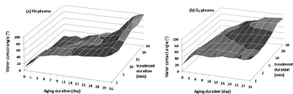
Fig. 4 Contact angle versus aging-time of PET surfaces plasma-treated at different durations, (a) He and (b) O 2 plasmas.
