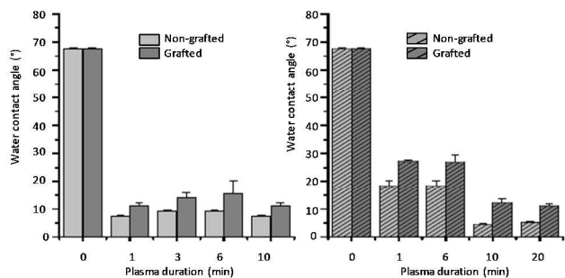
Fig. 6 Contact angle of PET films plasma-treated and grafted with Pluronic F108 versus plasma parameters (duration; (a) He and (b) O 2 plasmas.
