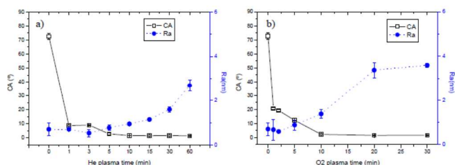
Fig. 1. Contact angle (empty squares) and R_a values (filled circles) of He (a) and O 2 (b) plasma-treated PET versus the duration.
