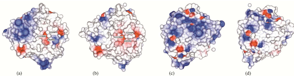
Figure 2. Change of electrostatic potential of the protein surface. Red areas have a negative potential, blue areas a positive potential, white areas are neutral. (a) subtilisin soaked in a CsCl salt aqueous solution; (b) in aqueous solution; (c, d) views at 180^\circ . Electrostatic potential of the protein surface were computed using CCP4MG 22 .
