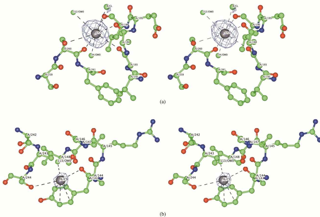
Figure 3. Stereo view of two representative Cs + ion binding sites. Atoms colored according to atom type: blue = N; red = O; green = C, grey = Cs). Anomalous difference Fourier map contour level at 4 \sigma . A) Cs site 2 coordination by carbonyls; b) Cs site 6 interacting with tyrosine ring.
