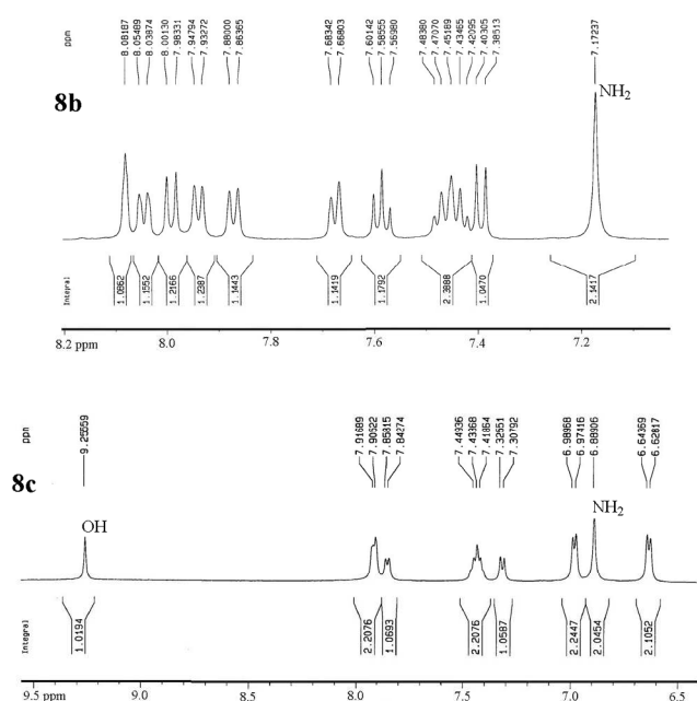
Figure 1. 500-MHz ^1\text{H-NMR} spectra of 8b and 8c in \text{DMSO-}d_6 for the aromatic proton resonances.
