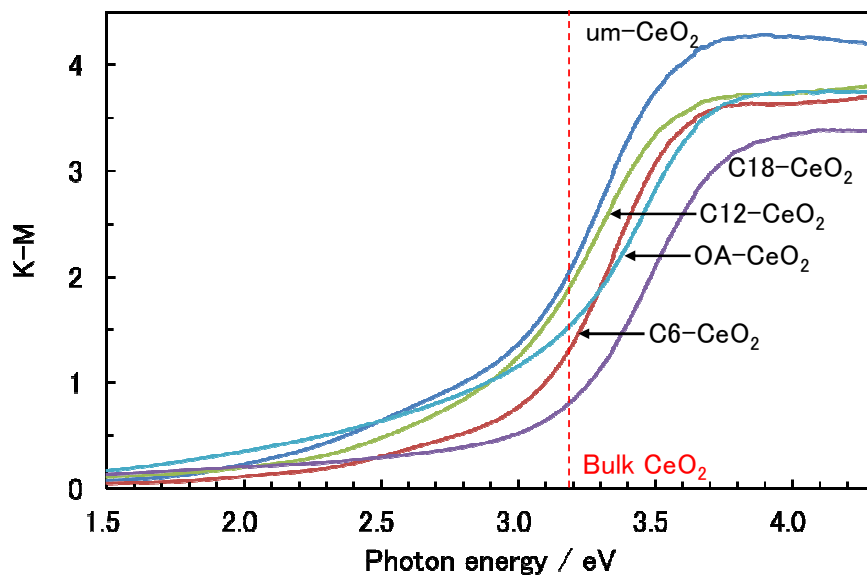
Figure 6. Typical UV-Vis powder diffuse-reflectance spectra of the products.
