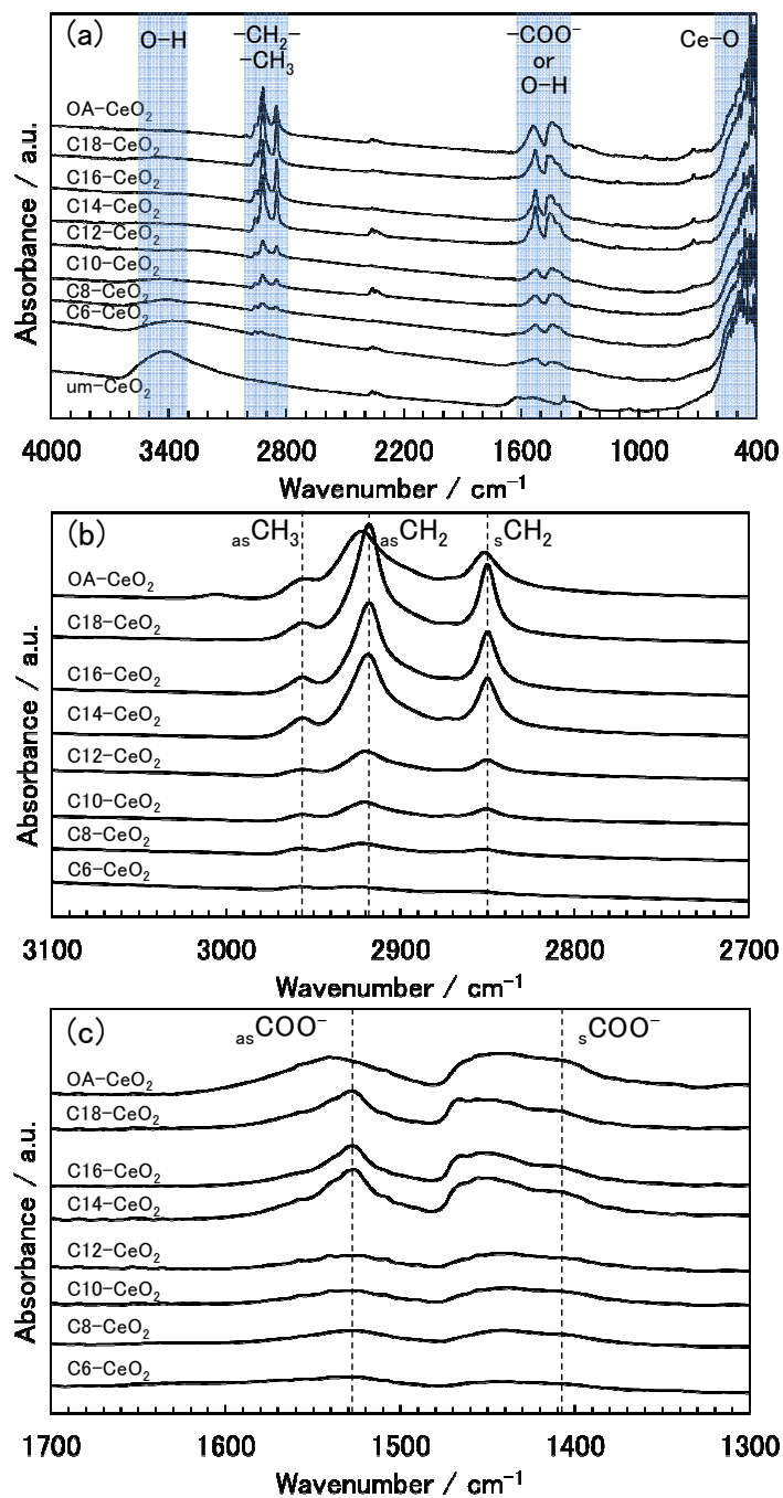
Figure 3. (a) FT-IR spectra of the CeO 2 nanoparticle products and evolution of the spectra enlarged in the ranges: (b) 3100–2700 cm -1 and (c) 1700–1300 cm -1 .
