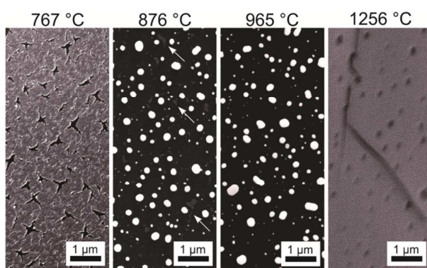
Figure 10. SEM-micrographs of rapidly cooled Pd-films annealed at the stated temperatures for 3 h.
