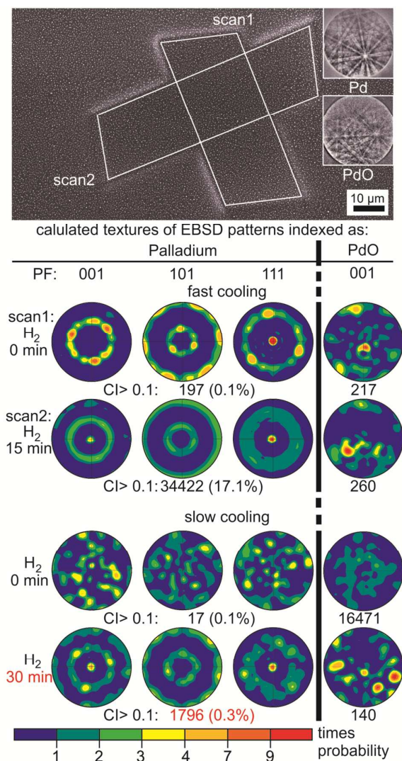
Figure 8. SEM-micrograph of Pd NP dewetted from a 18 nm thick Pd film by annealing for 3 h at 965 °C followed by fast cooling. EBSD-patterns of Pd and PdO are presented in the insets. EBSD-Scan 1 was performed directly after annealing while Scan 2 was performed after the sample was additionally flushed with H 2 gas for 15 min. Textures of Pd and PdO calculated from the Scans 1 and 2 as well as comparable scans obtained from a slowly cooled sample flushed with H 2 for 30 min are presented below along with the number of reliable data points (CI>0.1) contributing to the respective texture.
