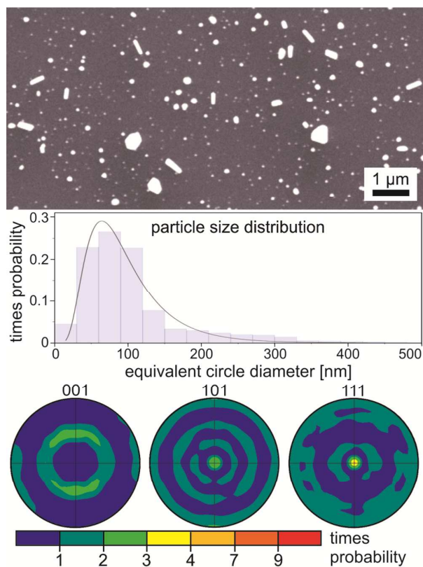
Figure 7. SEM-micrograph of Pt NP dewetted at 965 °C and pole figures of a texture calculated from an EBSD-scan performed on the surface. The elongated particles are nano rods protruding from the surface.
