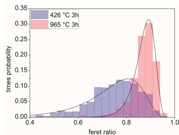
Figure 6. Feret Ratio of gold NP formed by dewetting at 426 and 965 °C.
