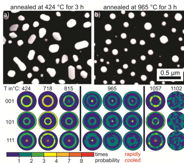
Figure 3. SEM-micrographs of gold NP dewetted on glass at a) 424 °C and b) 965 °C. Pole figures of textures calculated from EBSD-scans performed on layers dewetted at the stated temperatures visualize preferably occurring orientations.
