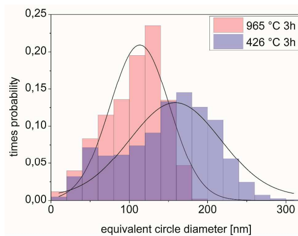
Figure 5. Equivalent circle diameter of gold NP formed by dewetting at 426 and 965 °C.
