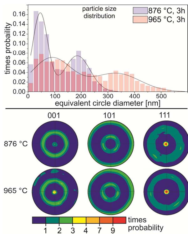
Figure 11. Temperature series of Pd layers annealed at the stated temperatures for 3h. SEM-micrographs feature surfaces from which EBSD-patterns could not be obtained. 001, 101 and 111 PFs of textures calculated from EBSD-scans performed on NPs dewetted from the Pd layers.
