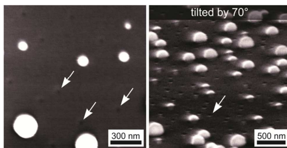
Figure 4. SEM-micrographs Au NP dewetted at 1102 °C for 3h.
