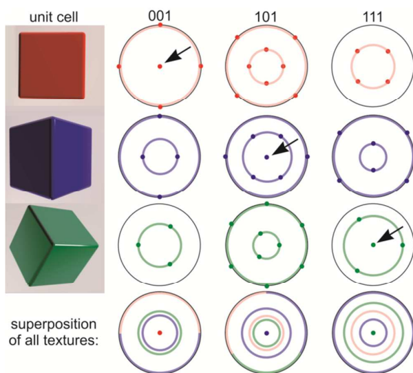
Figure 2. Orientations of a cubic unit cell and their poles in the respective pole figures. The rings indicate the result of a random rotation around the respective direction perpendicular to the image plane.
