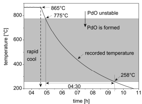
Figure 1. Measured temperature/time correlation of annealing a sample at 865 °C for 3 h followed by the slow cooling process. The rapid cooling procedure is indicated by the dashed line.
