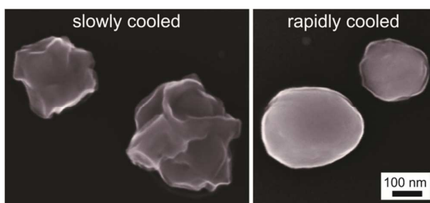
Figure 9. SEM-micrographs of dewetted Pd particles on the glass surface a) cooled slowly and b) cooled rapidly.
