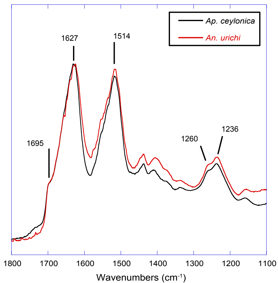
Fig. 4 FT-IR absorbance profiles comparing web spinner silks from the species Antipaluria urichi (red) and Aposthonia ceylonica (black). Spectra are virtually identical, emphasizing their remarkable similarity in structure.
