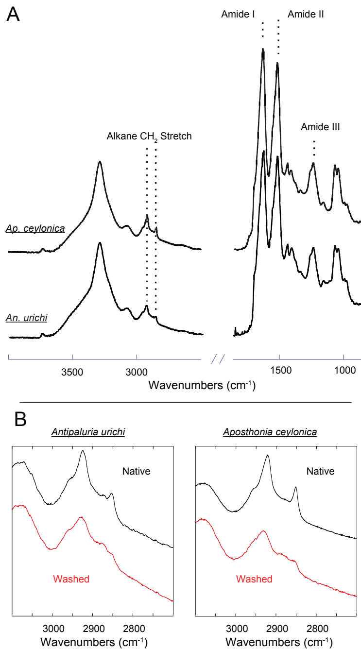
Fig. 3 A: FT-IR spectra of native Antipaluria urichi and Aposthonia ceylonica silk bundles. The strong amide I and II absorbances at 1625 and 1514 cm -1 , respectively, suggest that the protein core is predominantly \beta -sheet. B: Native webspinner silks (black) are compared to silks that were washed with 2:1 CHCl 3 :MeOH for 24 hours (red). Amide I, II and III bands remain unchanged (data not shown), but the alkane CH 2 symmetric and asymmetric stretches at 2850 and 2920 wavenumbers, respectively, drop approximately 50% in intensity after treatment. This is associated with the removal of a lipid or alkane-rich surface coating on the silk fibers.
