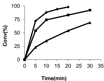
Figure 1: Effect of methanol content in water on ATH of 1a : 25% MeOH in water (▲), 50% MeOH in water (◆), 75% MeOH in water (■); 1a (0.5 mmol); HCOONa (2.5 mmol); Temp: 40°C, Solvent: 2 ml
