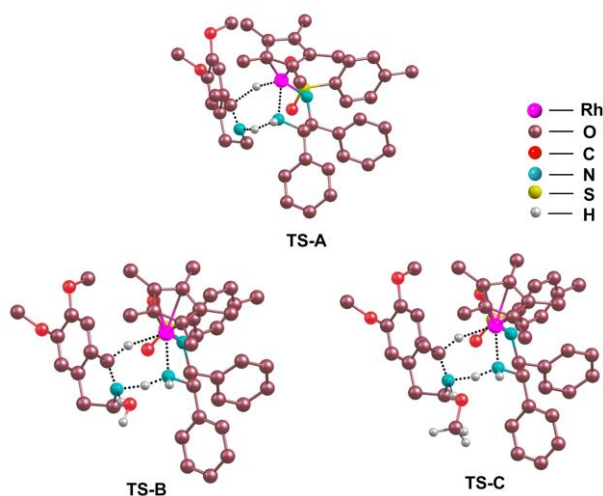
Figure 5: Proposed transition states without participation of solvent molecules ( TS-A ) and with participation of water ( TS-B ) and with participation of methanol ( TS-C ) (Hydrogen atoms have been omitted for the purpose of clarity)
