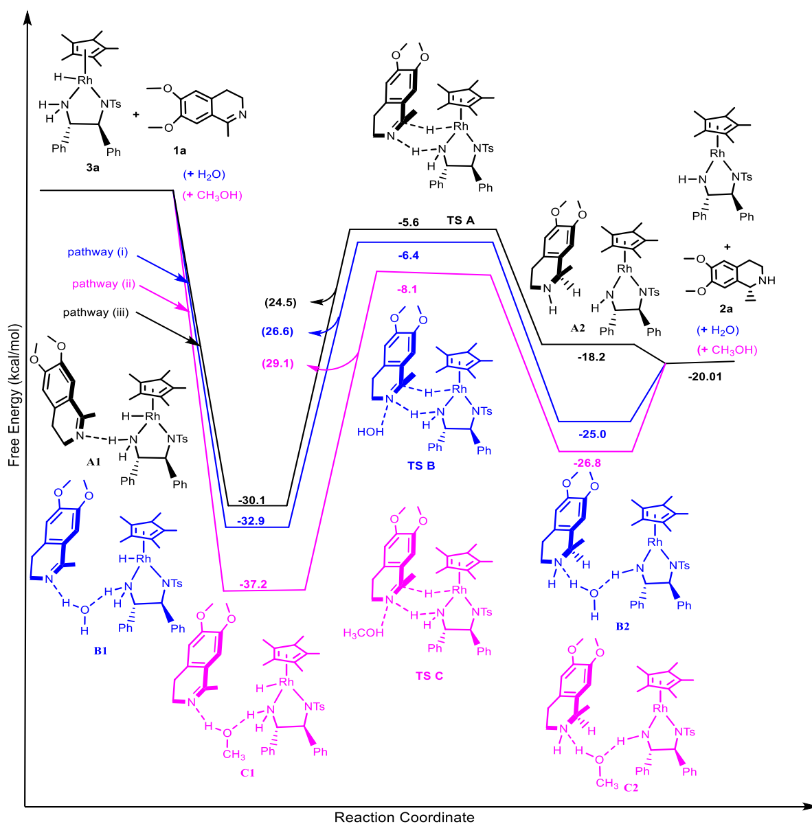
Scheme 2. Energy profiles for asymmetric transfer hydrogenation of imine calculated by the DFT method (energy difference in kcal/mol)
