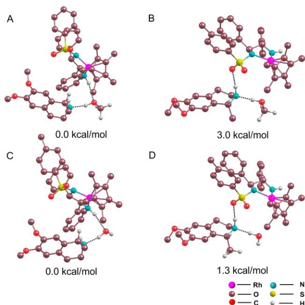
Figure 4: Optimized geometry structures of product; A: N-H of product 2a hydrogen bonding only with methanol, B: N-H of product 2a hydrogen bonding with sulfonyl oxygen of the TsDPEN ligand, C: N-H of product 2a hydrogen bonding only with water, D: N-H of product 2a hydrogen bonding with sulfonyl oxygen of the TsDPEN ligand; energy difference in kcal/ mol.
