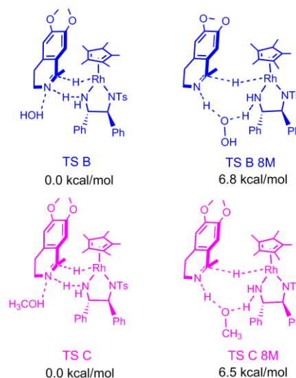
Figure 3. Structures of six membered and eight membered (8M) transition state for asymmetric transfer hydrogenation of imine (energy difference in kcal/mol)
