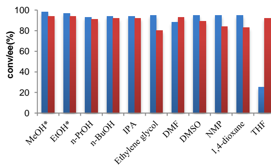
Figure 2: Co-solvent screening for ATH of 1a catalyzed by Rh-TsDPEN Conv(■), ee(■), Reactions were carried out on a 0.5 mmol scale in a 2ml Water/ Co-solvent(1:1, v/v) at 40°C, Time : 30 min, * Time: 20 min
