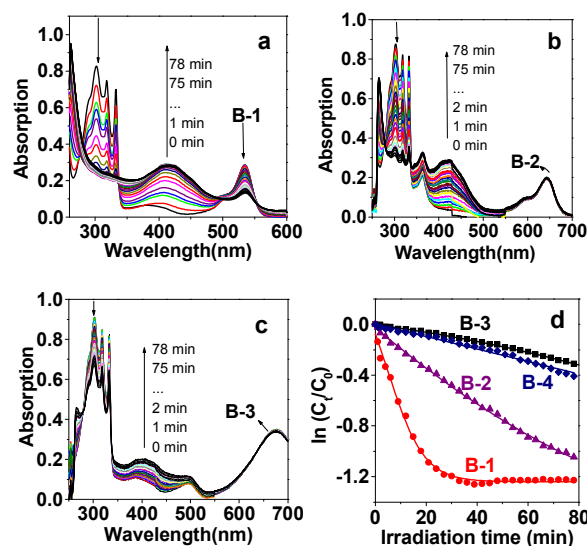
Figure 2 UV/Vis absorption spectral changes for the photooxidation of 1,5-DHN ( 1.0 \times 10^{-4} M) using SOPs (a) B-1 , (b) B-2 and (c) B-3 in DMF/H 2 O (5:1, v/v) mixed solvent, [SOP]= 5.0 \times 10^{-6} M (5% mol), 20 °C. Irradiated with 35 W xenon lamp ( 25 \text{ mW} \cdot \text{cm}^{-2} ). Light with wavelength shorter than 385 nm was blocked by 0.72 M NaNO 2 solution. (d) Absorption changes in the photooxidation of 1,5-DHN and plots of \ln(C_t/C_0) vs irradiation time.
