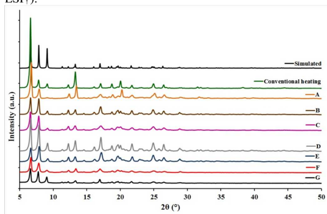
Fig. 4 XRD patterns of TMU-4 prepared by either conventional heating or sonochemical reaction (samples A-G). The data are in good agreement with the simulated pattern derived from the corresponding single-crystal structure data.
