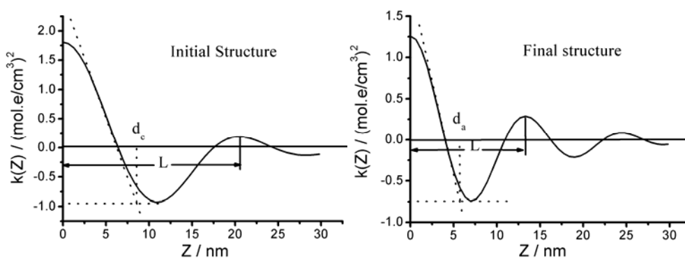
Figure 6. Curves of experimental correlation function K(Z) obtained for (a) initial structure and final structure of PEO- b -PLLA during isothermal crystallization at 40 °C after at 180 °C.
