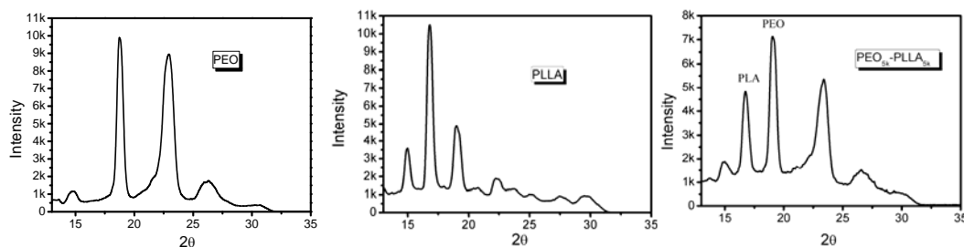
Figure 2. WAXS patterns of PEO, PLLA and the PEO-b-PLLA block copolymer.
