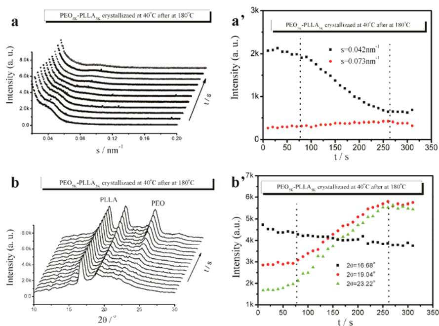
Figure 4. Simultaneous profiles and the integrated intensity I_{\text{int}} as a function of time obtained from SAXS (a, a') and WAXS (b, b') measurements during isothermal crystallization of PEO-b-PLLA at 40 °C.
