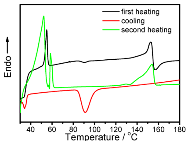
Figure 1. DSC curves for PEO-b-PLLA block copolymer
