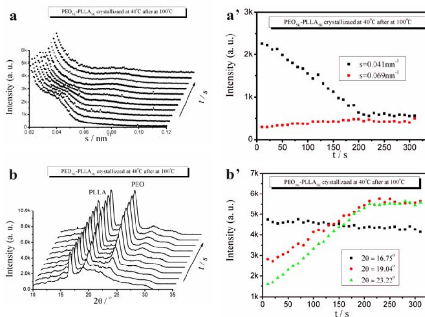
Figure 8. Simultaneous profiles and the integrated intensity I_{\text{int}} as a function of time obtained from SAXS (a, a') and WAXS (b, b') measurements during isothermal crystallization of PEO-b-PLLA at 40 °C after at 100 °C.
