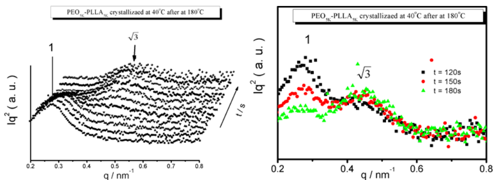
Figure 5. Time related Iq^2 versus q of PEO-b-PLLA crystallized at 40^\circ\text{C} during isothermal crystallization.
