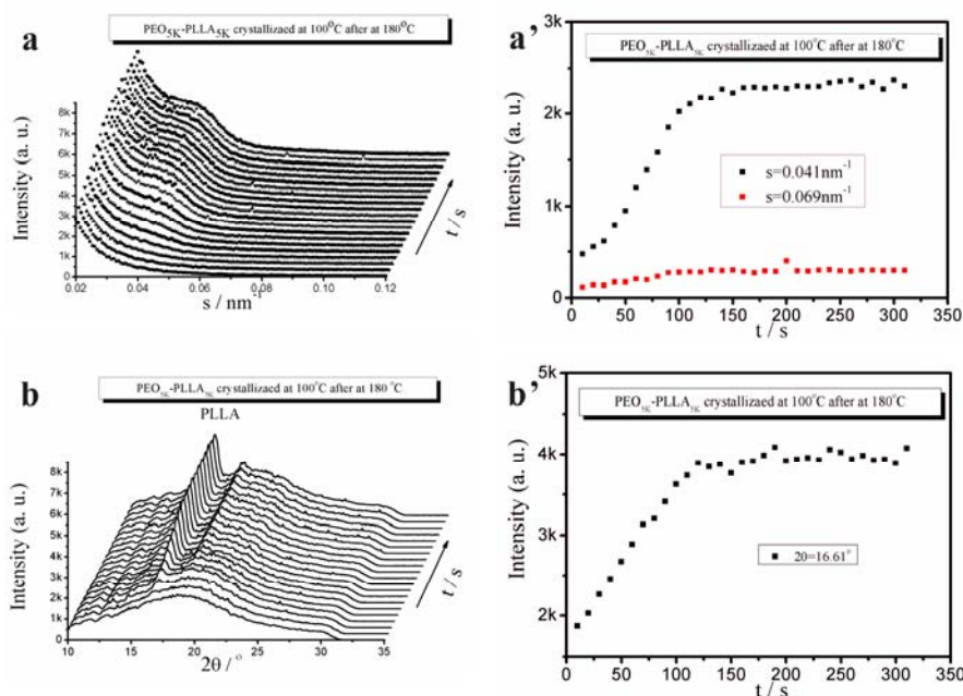
Figure 7. Simultaneous profiles and the integrated intensity I_{\text{int}} as a function of time obtained from SAXS (a, a') and WAXS (b, b') measurements during isothermal crystallization of PEO-b-PLLA at 100 °C. It is reported that the peaks corresponding to the lamellar repeat were revealed in the supercooled melt (by SAXS) prior to the observation of three-dimensional crystal ordering (by WAXS), and the lag time ( t_{\text{WAXS}} - t_{\text{SAXS}} ) reduces with decreasing the crystallization temperature or increasing the degree of supercooling. Wang et al. reported the lag time is attributed to the detection limits of SAXS and WAXS. It is meaningless that only compare the first increase of the SAXS and WAXS intensities to confirm the appearance of initial crystalline phase because the detection limits of SAXS and WAXS are different. They considered that the crystallinity in the early stages is so low that the WAXS technique can not to detect it. But the crystallinity can be readily detectable by SAXS as long as the contrast between the constituting phases is sufficient and the length scale is within the detectable range. 27 However, the experiment data we obtained for PEO-b-PLLA and PEO-b-PCL block copolymers were not consistent with theirs as shown in Figure 4 and reference 24. Our results obtained from crystalline-crystalline diblock copolymers via simultaneous SAXS/WAXS measurements indicate that SAXS and WAXS could detect polymer crystallization process with different scales simultaneously. In other words, the lamella and crystallite structural transitions of block copolymer with double crystalline blocks can be measured during the crystallization processes of the two blocks. The detail of the structural transitions can be investigated and analyzed from the crystallization of the block copolymers.
