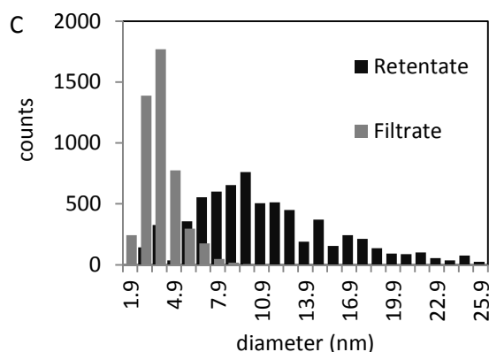
Figure 7. TEM micrographs showing the Ag-gly sample after filtration through the 100 KDa cellulose membrane: A) retentate and B) filtrate. C) Histogram showing the size distributions of the retentate and filtrate samples.
