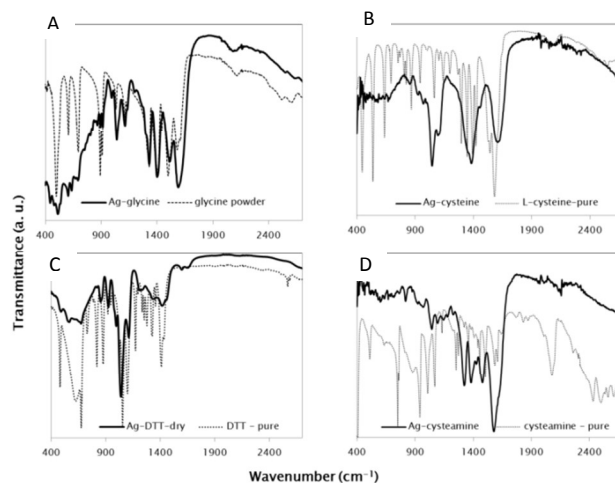
Figure 3. FT-IR spectra of the dried concentrates of A) Ag-glycine, B) Ag-cysteine, C) Ag-DTT and D) Ag-cysteamine. Spectra of pure ligands are presented in the dotted traces.
