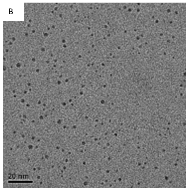
Figure 6. TEM micrographs and table showing the aggregation of Ag-glycine NPs upon increasing the ionic strength by NaCl.
