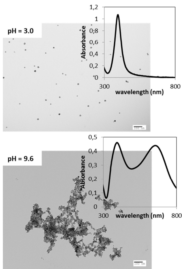
Figure 5. TEM micrographs of Ag-cysteamine in acidic and basic environments with their corresponding extinction spectra.
