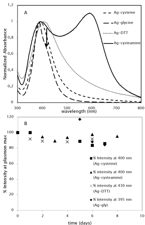
Figure 2. A) Absorption spectra of the silver colloids prepared with the four types of ligands: glycine, cysteine, DTT and cysteamine. The spectra were normalized to the absorbance value at \lambda_p of each type of ligands. B) Change in % plasmon intensity for AgNPs capped with the four types of ligands with time.
