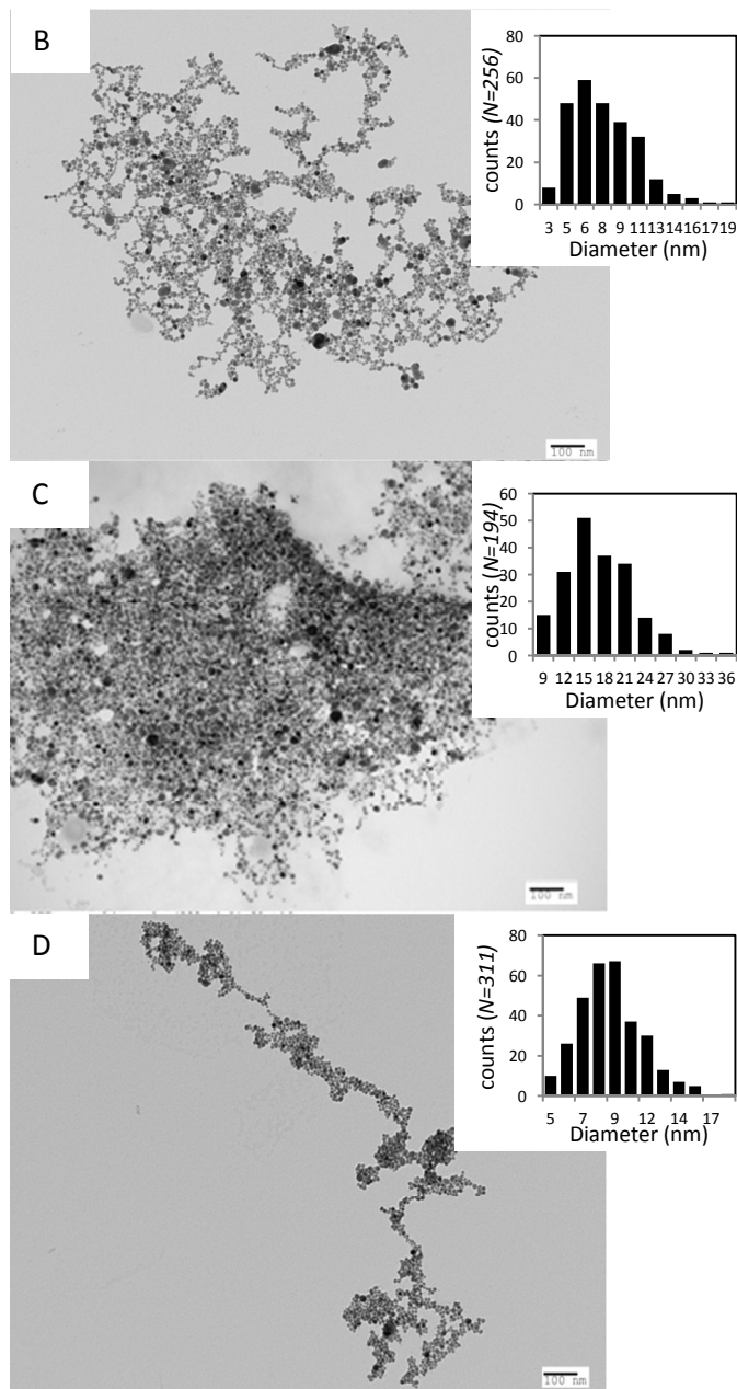
Figure 4. TEM micrographs of A) Ag-glycine; B) Ag-cysteine; C) Ag-DTT; D) Ag-cysteamine. Insets are the size distribution histograms with the total number of NPs analysed indicated.
