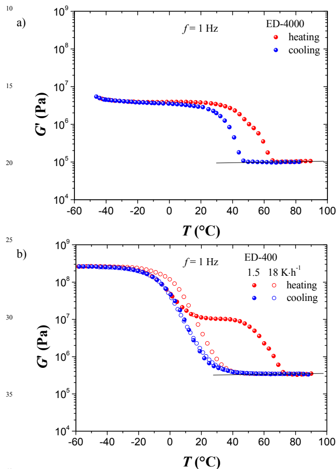
Fig. 3 Temperature dependence at f = 1 Hz of G' for a) the elastomer ED-4000 (long primary amino-terminated polyetheramine) at dT/dt = 3 K·h -1 , and for b) the elastomer ED-400 (short primary amino-terminated polyetheramine) at dT/dt = 1.5 and 18 K·h -1 . The solid lines represent the classical k_B T behaviour.
