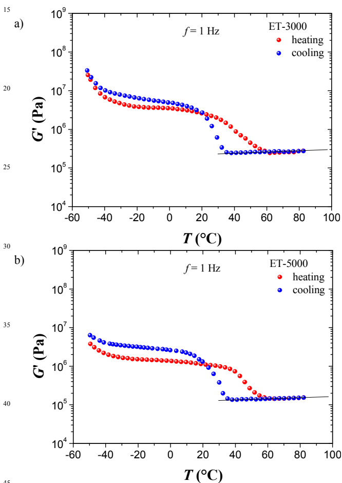
Fig. 7 Temperature dependence at f = 1 Hz of G' for the elastomers containing primary amino-terminated polyetheramines at dT/dt = 3 K·h -1 : a) the elastomer ET-3000, and b) the elastomer ET-5000. The solid lines represent the classical k_B T behaviour.
