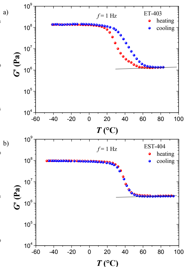
Fig. 6 Temperature dependence at f = 1 \text{ Hz} of G' for a) the elastomer ET-403 (primary amino-terminated polyetheramine which forms disubstituted urea groups with bidentated hydrogen bonds) at dT/dt = 3 \text{ K}\cdot\text{h}^{-1} , and for b) the elastomer EST-404 (secondary amino-terminated polyetheramine which forms trisubstituted urea groups without bidentated hydrogen bonds) at dT/dt = 3 \text{ K}\cdot\text{h}^{-1} . The step variation comes from the contribution of the glass transition for EST-404, and from the simultaneous contribution of the glass transition and of the hydrogen bonds for ET-403. For both elastomers, the solid lines represent the classical k_B T behaviour.
