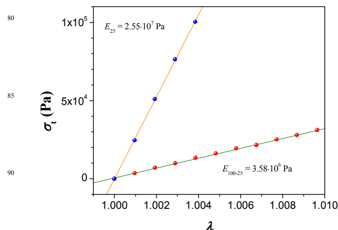
Fig. 4 Stress-strain curves for the elastomers ED-400 at T = 25 °C after annealing the sample at 100 °C (●) and directly measured from the synthesis (●). The solid straight lines are the fits of the data belonging to the purely elastic region.
