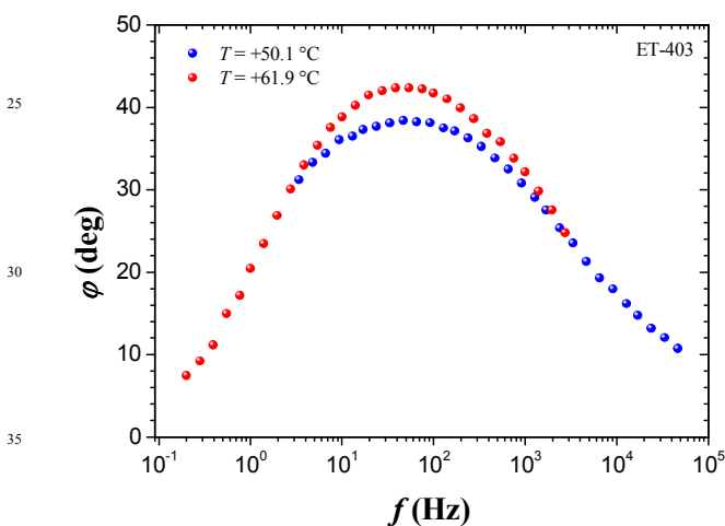
Fig. 15 Behaviour of the loss angle \phi as a function of frequency for the elastomer ET-403. The temperatures of measurement are T = +50.1 °C and +61.9 °C. The last curve has been shifted along the frequency axis to show that the time-temperature superposition method does not work.
