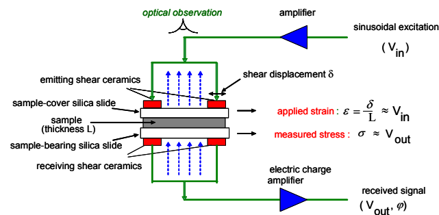
Fig. 1 Block diagram of the piezoelectric rheometer.
