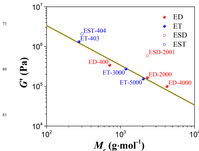
Fig. 11 Log-log plot of the shear storage modulus G' as a function of the segmental molecular weight M_c for the eight elastomers at T = 80 °C, where the measurements correspond to the elastic plateau of the chemical network. For each series ED and ET, the data are consistent with the relationship G' \propto M_c^{-1} represented by the solid straight lines. The fact that the data of the elastomers EST-404 and ESD-2001 are not on the solid straight lines associated with the ED and ET series shows that the architecture of these two elastomers strongly differs from that of the elastomers of each series.
