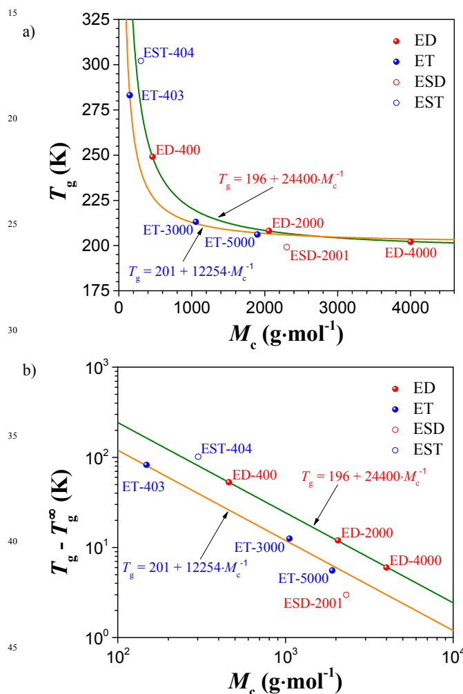
Fig. 10 a) linear-linear plot and b) log-log plot for the variation of the glass transition temperature T_g as function of the segmental molecular weight M_c for the eight elastomers, showing for each series ED and ET that the short polymers raise the glass transition temperature due to the low mobility of the polymer segments between crosslinking points. T_g^\infty is the extrapolated glass transition temperature at infinitum segmental molecular weight from the Fox-Flory empirical model. The elastomers ESD-2001 and EST-404 do not follow the Fox-Flory laws for the ED and ET series because of their different architecture.
