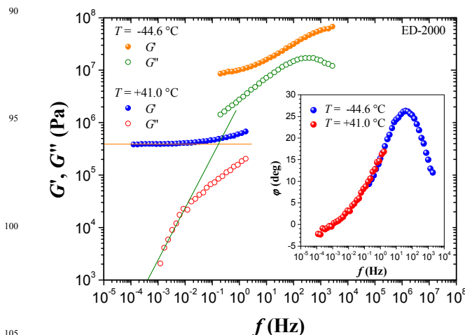
Fig. 14 Behaviour of G' and G'' as a function of the frequency for the elastomer ED-2000 showing that the time-temperature superposition method does not work. The shift factor corresponds to the one used to obtain the master curve for the loss angle \phi , represented in the insert of the figure. A shift factor of 17 along the G -axis would be needed to obtain a master curve for G' and G'' .
