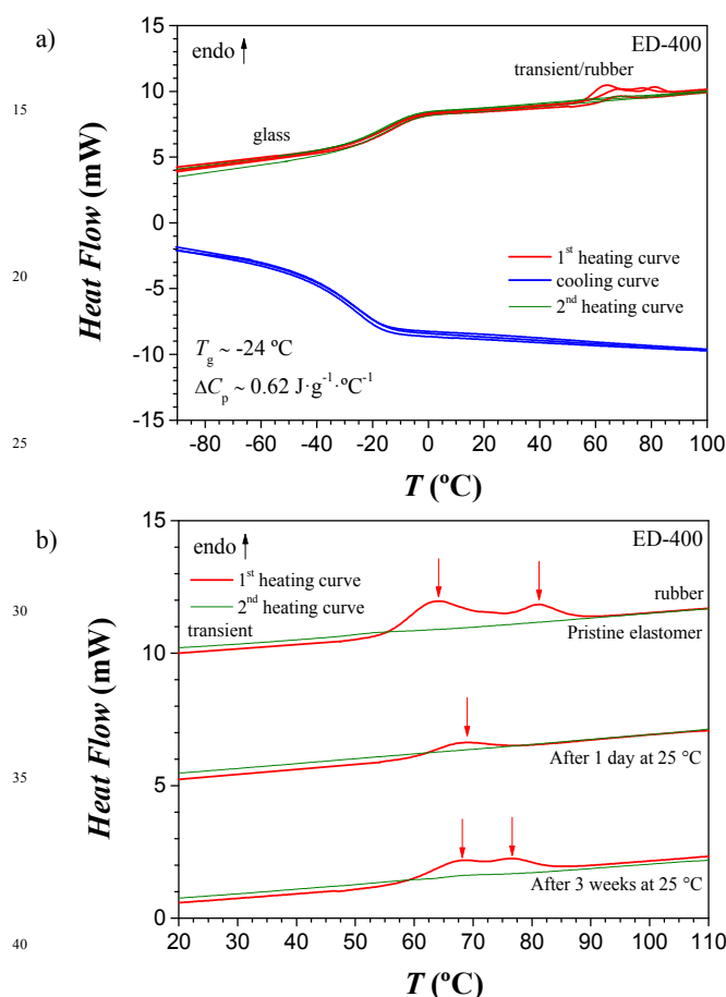
Fig. 5 a) Different heating and cooling DSC thermographs for the elastomers ED-400 at 20 \text{ K}\cdot\text{min}^{-1} showing the presence of enthalpic peaks. b) Zoom in on the heating thermographs on the same elastomer ED-400 sample directly after the synthesis ( T_{\text{HB}} \sim 64 & 81 °C, \Delta H_{\text{HB}} \sim 5.2 \text{ J}\cdot\text{g}^{-1} ), after 1 day ( T_{\text{HB}} \sim 68 °C, \Delta H_{\text{HB}} \sim 1.3 \text{ J}\cdot\text{g}^{-1} ) and 3 weeks later ( T_{\text{HB}} \sim 68 & 76 °C, \Delta H_{\text{HB}} \sim 3.2 \text{ J}\cdot\text{g}^{-1} ). Note: the second heating curves do not show any enthalpic peak, indicating that the hydrogen bonds have not enough time to reform during the experimental time scale.
