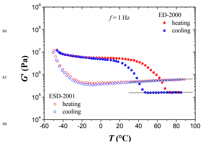
Fig. 2 Comparison between the temperature dependence at f = 1 Hz of G' for the elastomer ED-2000 (primary amino-terminated polyetheramine which reacts forming disubstituted urea groups with bidentated hydrogen bonds) and the elastomer ESD-2001 (secondary amino-terminated polyetheramine which reacts forming trisubstituted urea groups without bidentated hydrogen bonds) both at dT/dt = 3 \text{K}\cdot\text{h}^{-1} . The data for the elastomer ED-2000 show the presence of a transient network associated with the formation and breaking of hydrogen bonds. The solid lines represent the classical k_{\text{B}}T behaviour.
