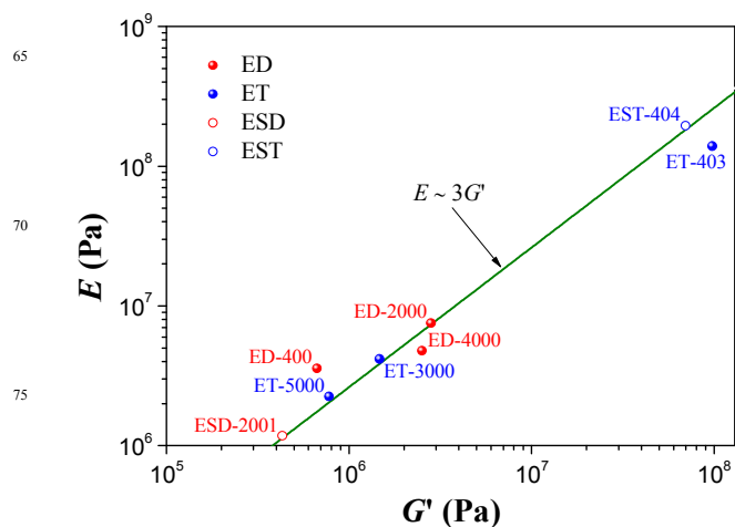
Fig. 9 E versus G' at T = 25 °C for the various elastomers studied. The E and G' measurements were taken after cooling the elastomers. The data are consistent with the relationship E = 3G' represented by the solid straight line, except for elastomers ED-400 and ET-403, for which both glass transition effects and hydrogen bonds contribute to G' at this temperature.
