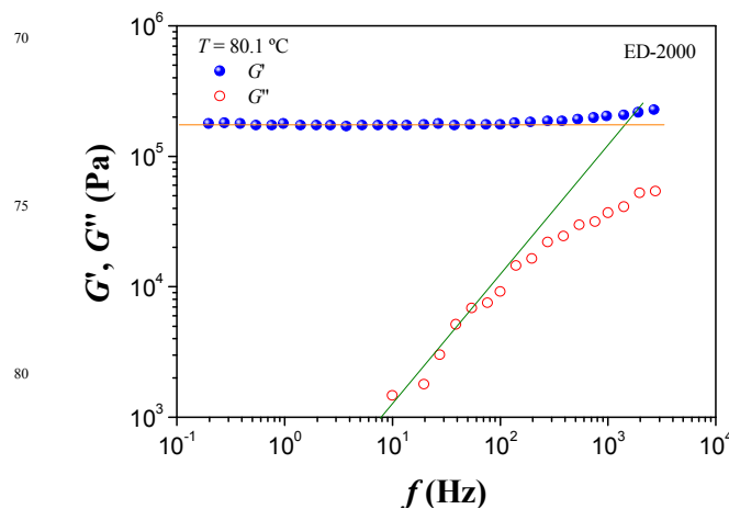
Fig. 13 Behaviour of G' and G'' as a function of frequency for the elastomer ED-2000 at a temperature located above the temperature of formation of the transient elastomer showing that the low frequency response of the material is that of a chemically crosslinked elastomer and not that of a long chain polymer.
