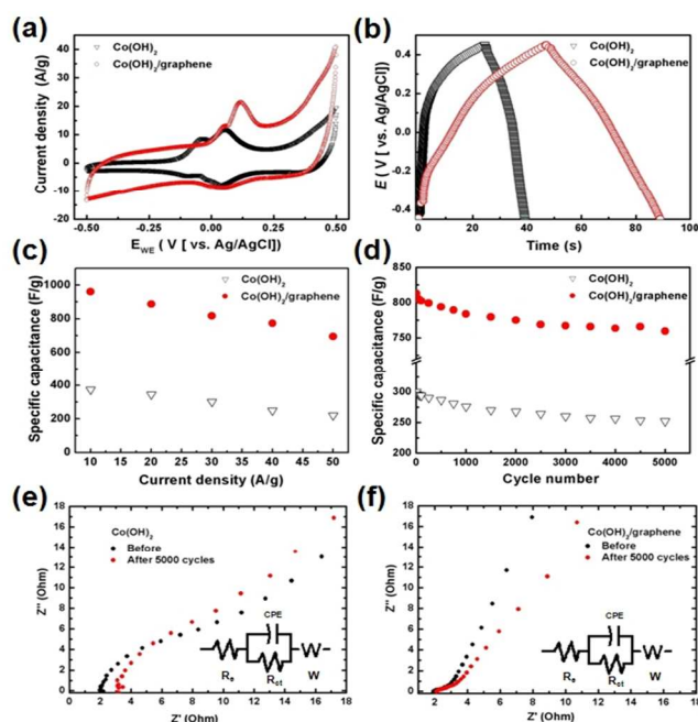
Fig. 4 (a) Cyclic voltammetry (CV) curves of Co(OH) 2 and Co(OH) 2 /graphene at 100mV/s in 2 M KOH solution. (b) Galvanostatic charge/discharge behaviors of Co(OH) 2 and Co(OH) 2 /graphene electrodes at a constant current density 10 A/g in 2 M KOH solution. (c) Specific capacitance of Co(OH) 2 and Co(OH) 2 /graphene electrodes in the range of current density 10 to 50 A/g. (d) Cycling life of Co(OH) 2 and Co(OH) 2 /graphene at a constant current density 30 A/g in 2 M KOH solution. Nyquist plots of (e) the Co(OH) 2 and (f) Co(OH) 2 /graphene electrode before/ after 5000 cycles in the 2 M KOH solution at a current density of 10 A/g.
