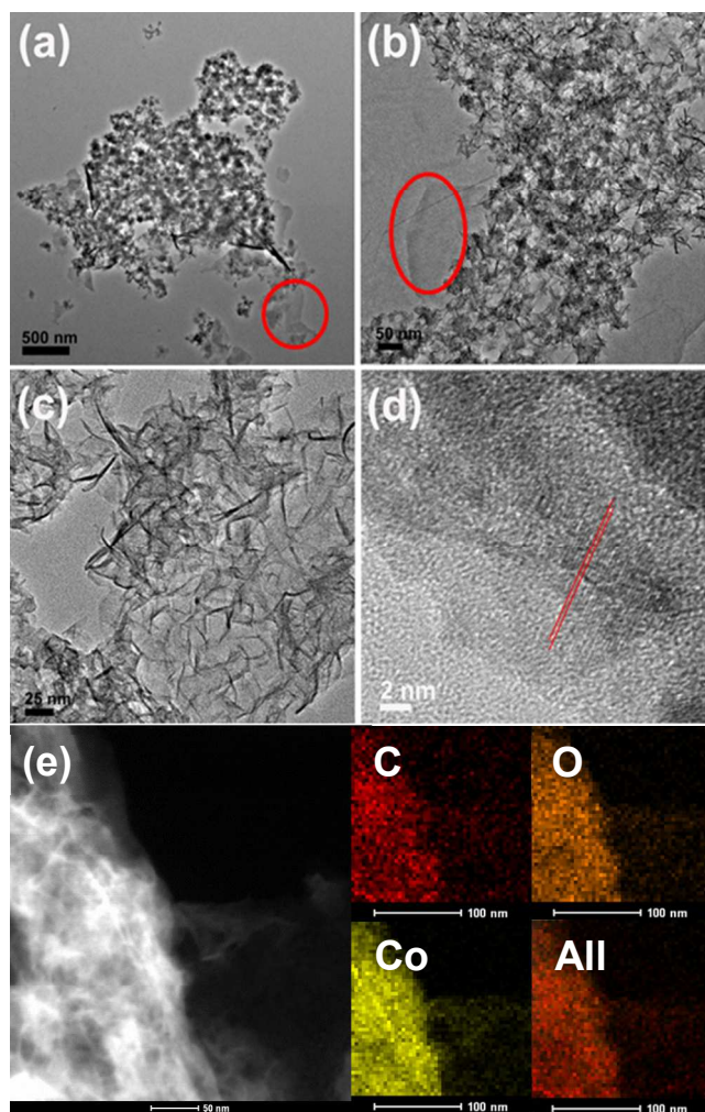
Fig.2 TEM images of \text{Co(OH)}_2 /graphene nanocomposites. Red circles in (a) and (b), show graphene. (c), (d) magnified image of \text{Co(OH)}_2 nanosheets on graphene Lattice distance of \text{Co(OH)}_2 is 0.236 nm. (e) HAADF-STEM mapping images of \text{Co(OH)}_2 nanosheets on graphene.
