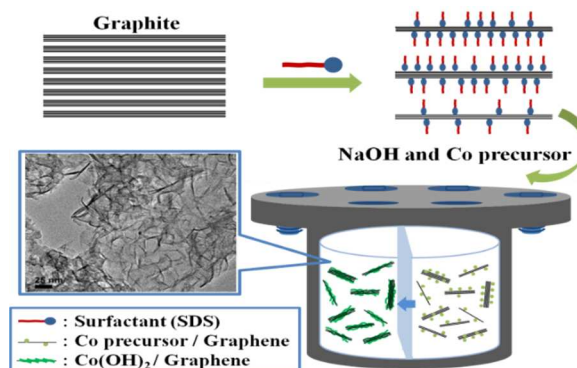
Fig. 1 Synthesis of \text{Co(OH)}_2 /graphene composites from graphite.
