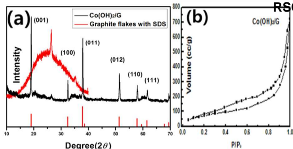
Fig. 3 (a) XRD patterns of Co(OH) 2 /graphene nanocomposites and graphene flakes functionalized SDS. Red peaks are the reference of Co(OH) 2 . (JCPDS No. 30-0443) (b) Nitrogen adsorption/desorption isotherms distribution of Co(OH) 2 /graphene nanocomposites.
