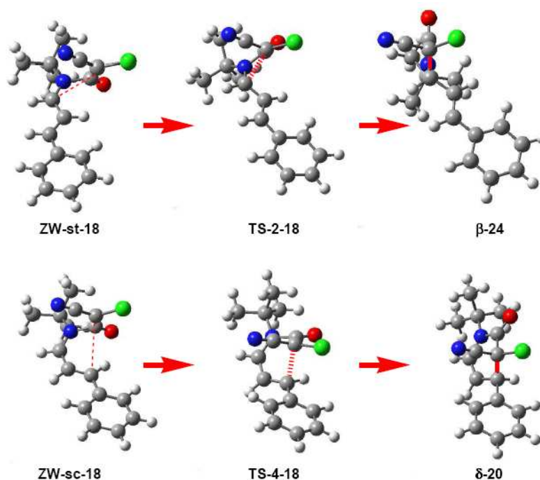
Figure 3. Geometrical changes along the formation of \beta -lactam \beta -24 and \delta -lactam \delta -20. While \beta -24 presents a trans diastereoisomeric relation of the CN group relative to the chain, \delta -20 presents a cis disposition of the CN group relative to the phenyl substituent.
