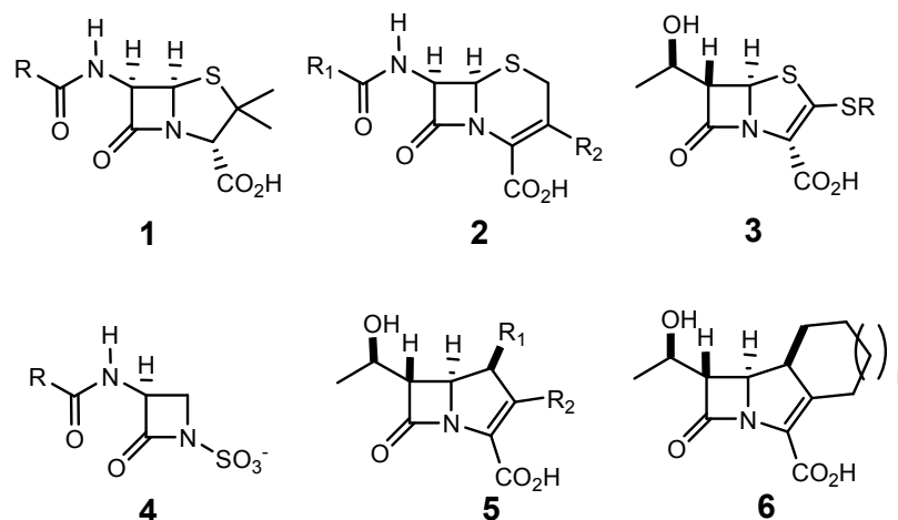
Scheme 1. Some representative structural classes of \beta -lactam antibiotics.
