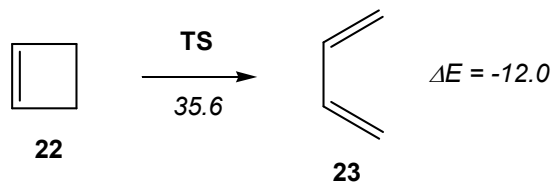
Scheme 5. Electrocyclic aperture of cyclobutene 22 . Energies are in kcal/mol.
