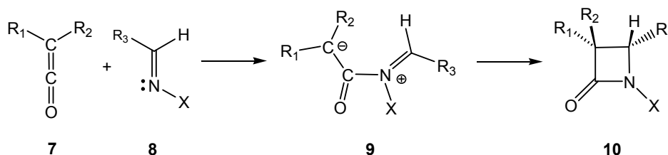
Scheme 2. Mechanism of the Staudinger reaction.
