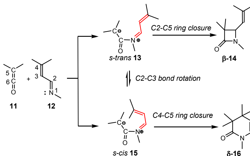
Scheme 3. Reactions between ketenes 11 and \alpha,\beta -unsaturated imines 12 .
