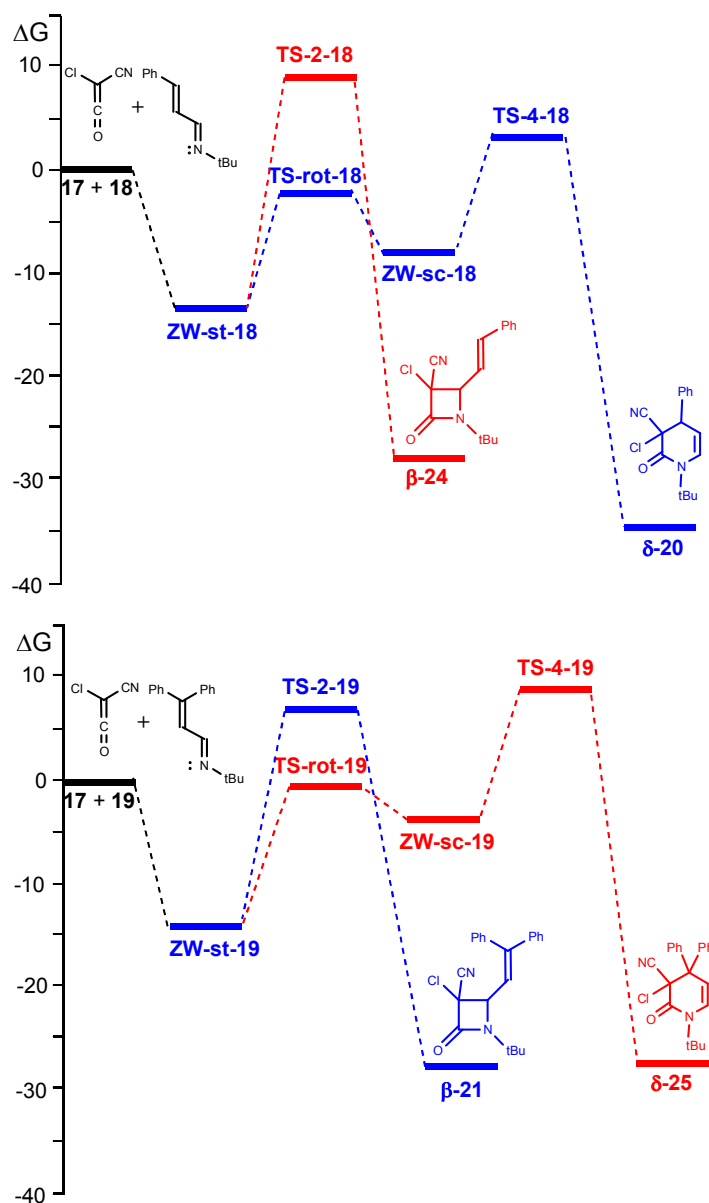
Figure 1. MPWB1K/6-311G(d,p) free energy profiles (in kcal/mol) in DEE of the reactions of CCK 17 with UIs 18 , up, and 19 , down. The most favourable reactive channels associated with the formation of lactams δ-20 and β-21 are given in blue.
