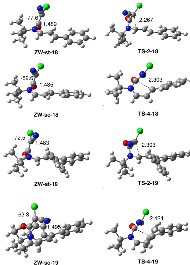
Figure 2. Structures of the ZW intermediates and TSs associated with the formation of \beta -lactams and \delta -lactams in the reactions of CCK 17 with UIs 18 and 19 . The distances are given in Angstroms, while the dihedral angles are given in degrees.
