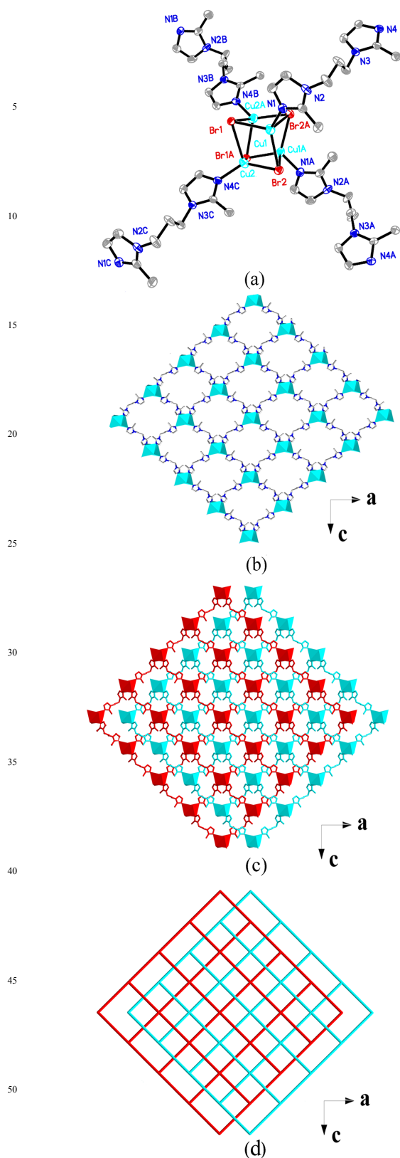
Fig. 1 (a) Molecular structure of 1 containing a cubane [\text{Cu}_4\text{Br}_4] cluster. Symmetry codes: (A) 2 - x, 2 - y, z ; (B) 1 - x, 2 - y, z - 1 ; (C) 1 + x, y, z - 1 . (b) A single 2D layer structure of 1 . (c) View of the 2-fold interpenetrating 3D framework of 1 . (d) Topological representation of the 2-fold interpenetration in 1 .
